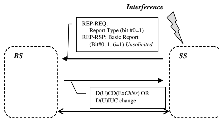
Figure h3—Link level representation of DCS operation
