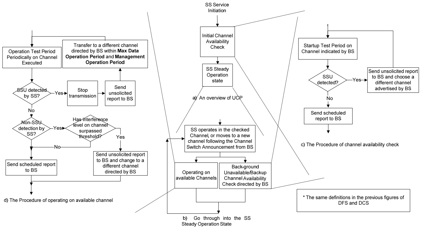
Figure hucp1 Flowchart showing generic operation of UCP at the SS in bands with SSUs and non-SSUs
