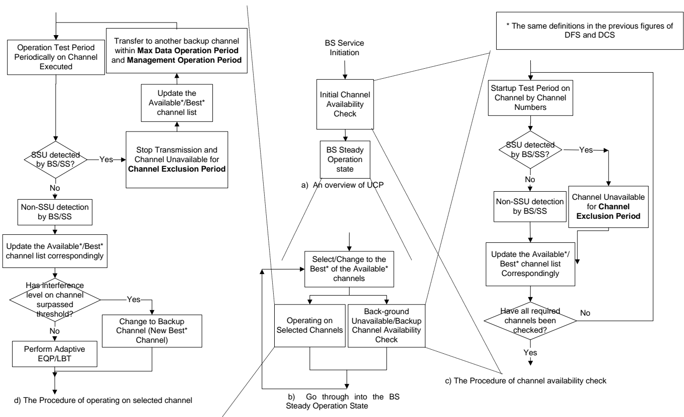
Figure hcup1 Flowchart showing generic operation of UCP at the BS in bands with SSUs and non-SSUs
