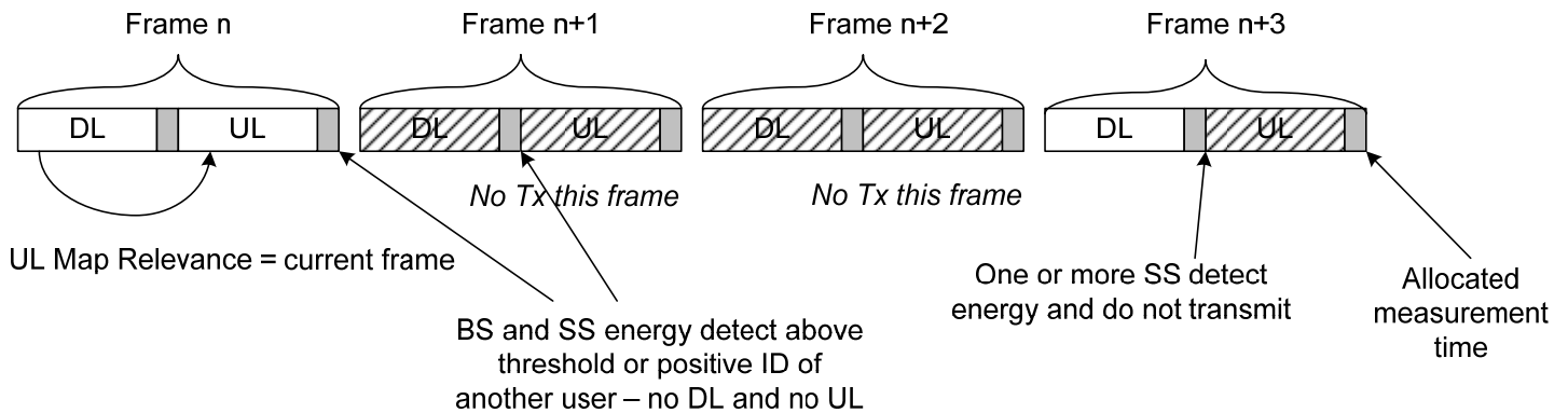
Figure h7— listen-before-talk LBT [Note: revised figure]
