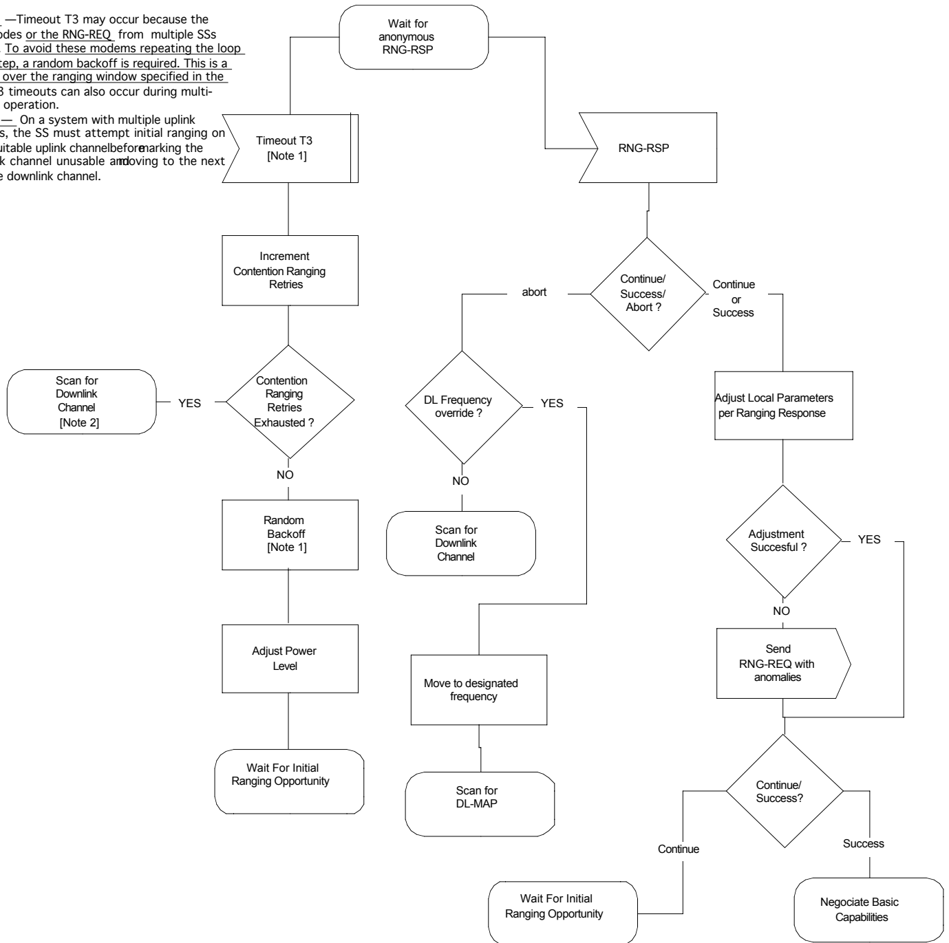
Figure 86 – CDMA Initial Ranging – SS (part 2)
