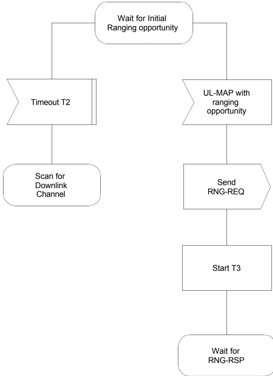
Figure 60 – Initial Ranging – SS (part 1)
