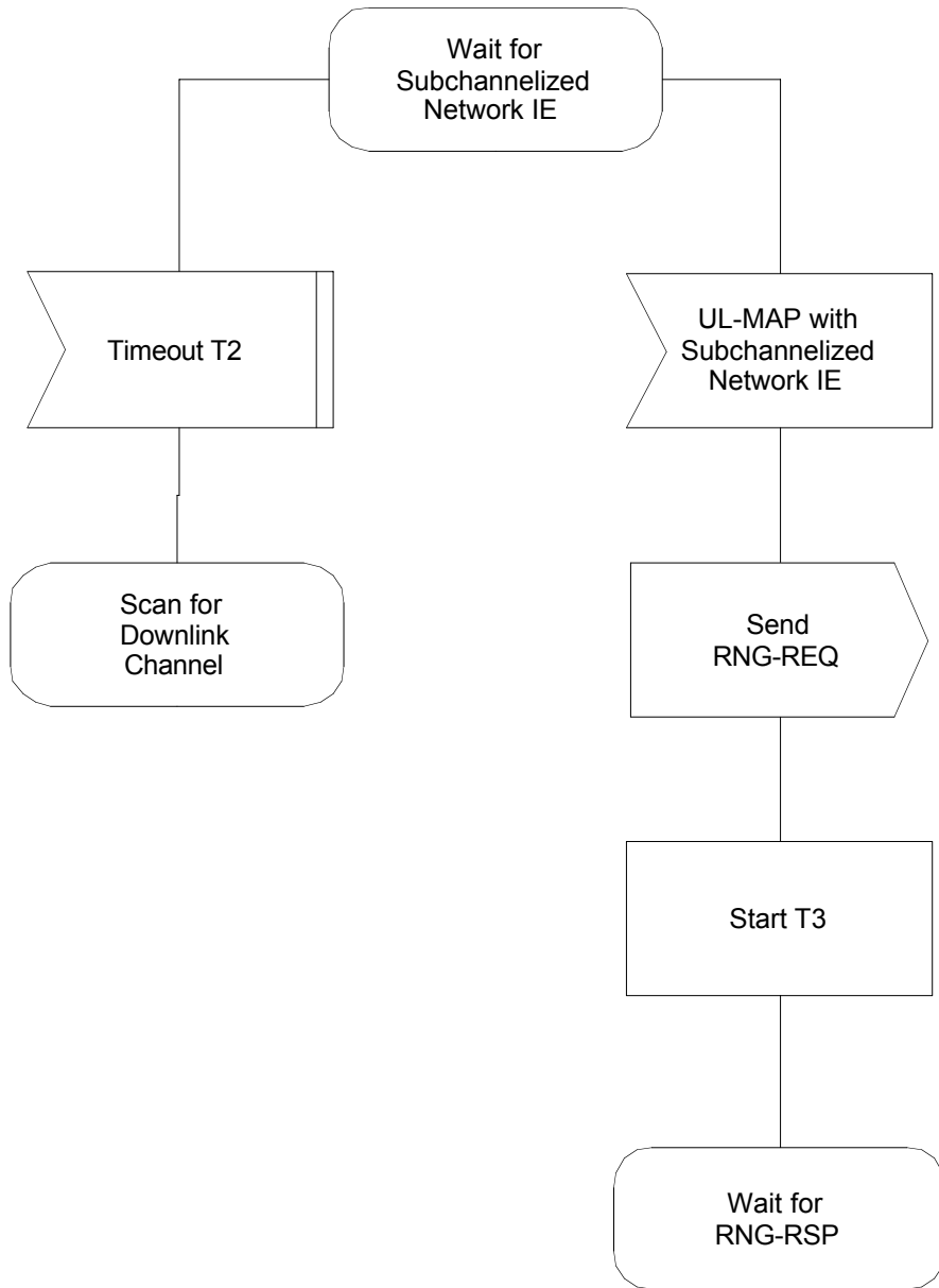
Figure 210b – Subchannelized Initial Ranging – SS (part 1b)
