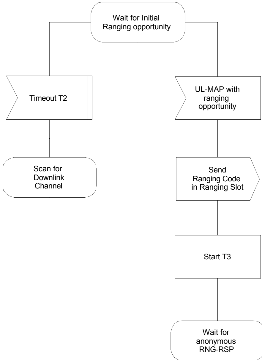
Figure 85 – CDMA Initial Ranging – SS (part 1)
