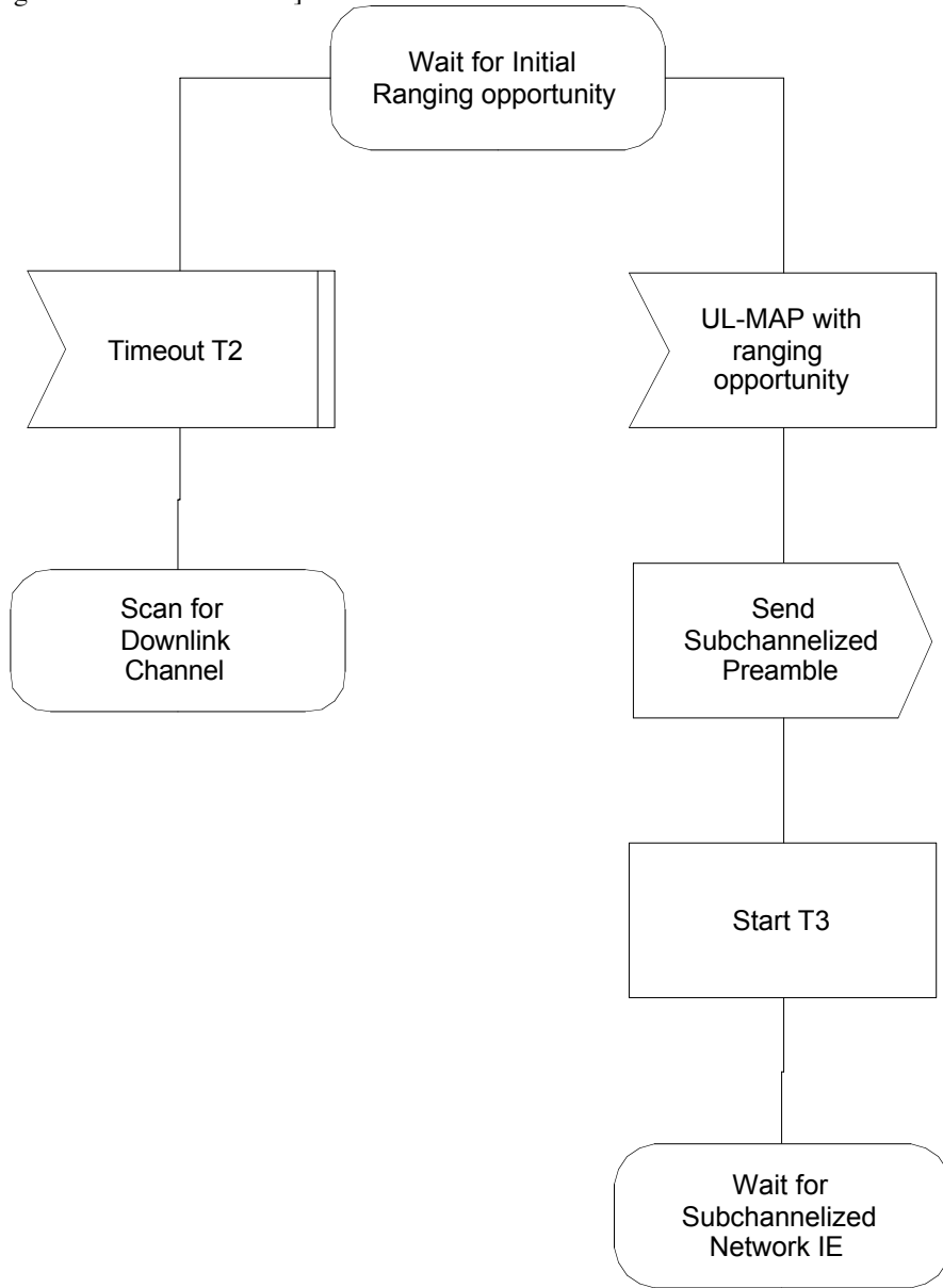
Figure 210a – Subchannelized Initial Ranging – SS (part 1a)
