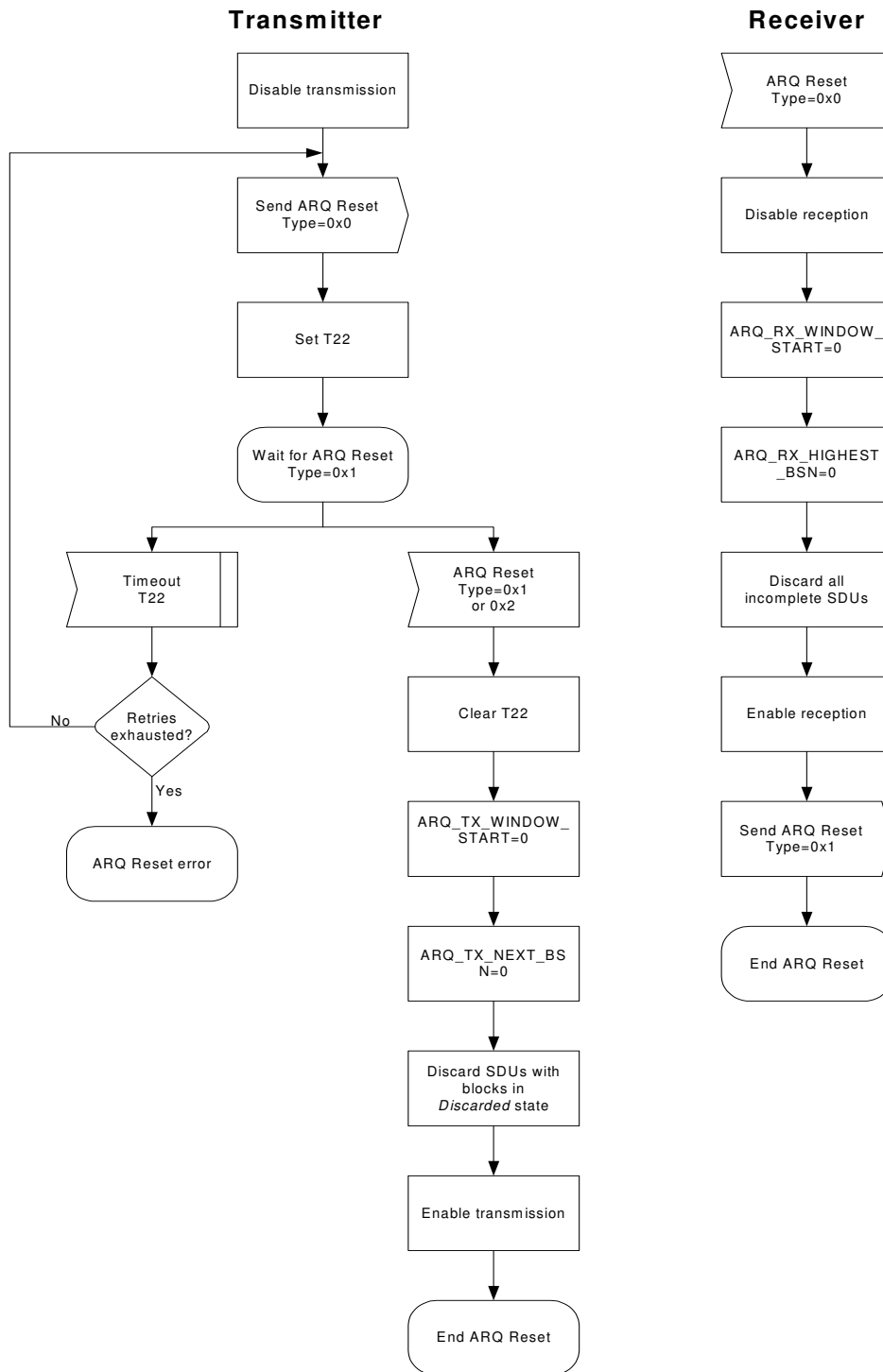
Figure 34-ARQ Reset message dialog-transmitter initiated
