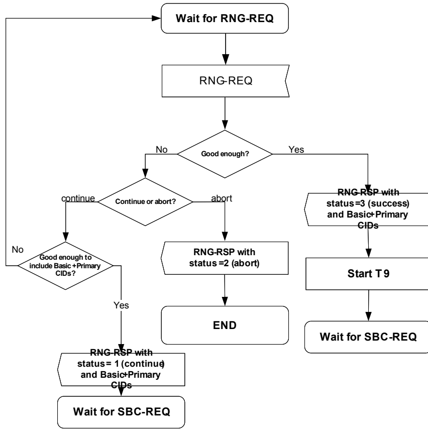
Figure 87b – Handle RNG-REQ (OFDMA PHY only)
