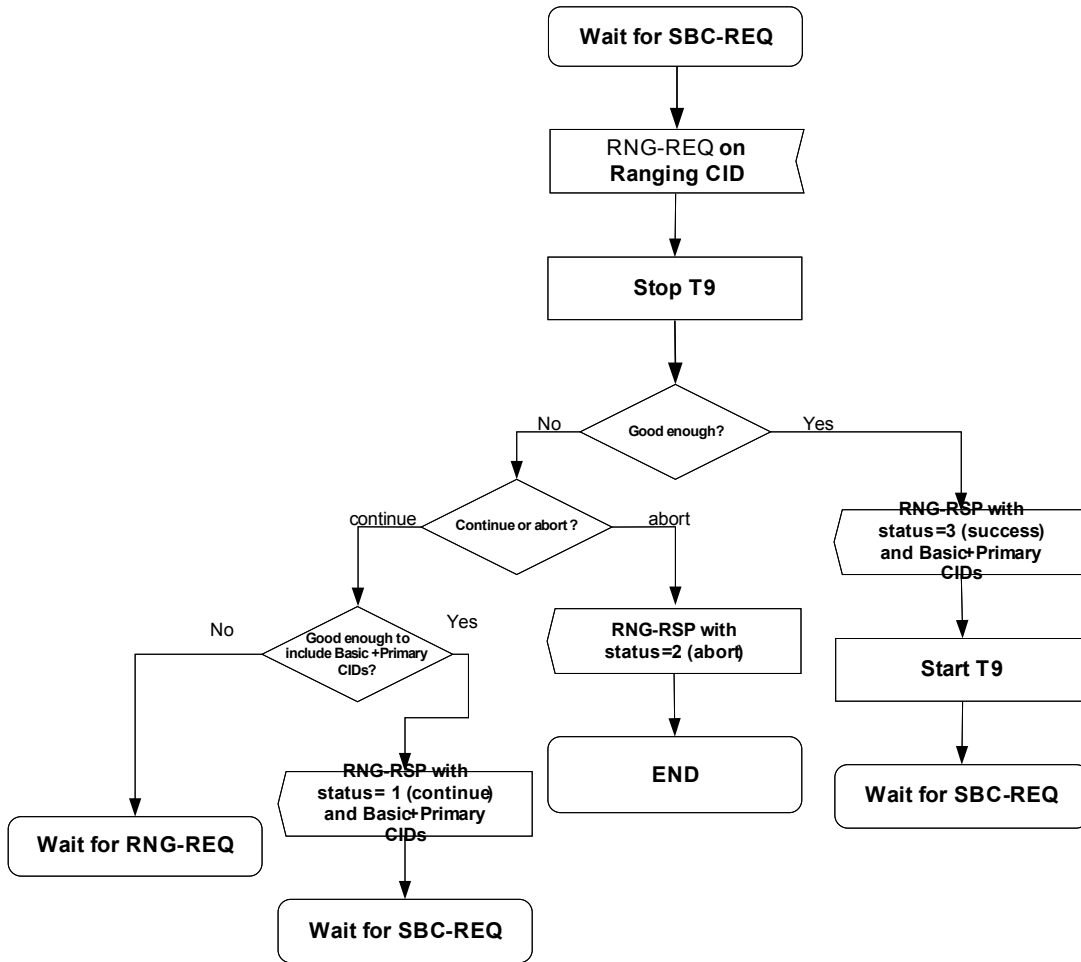
Figure 87c – Handle RNG-REQ retransmission after MS T6 Timeout (OFDMA PHY only)
