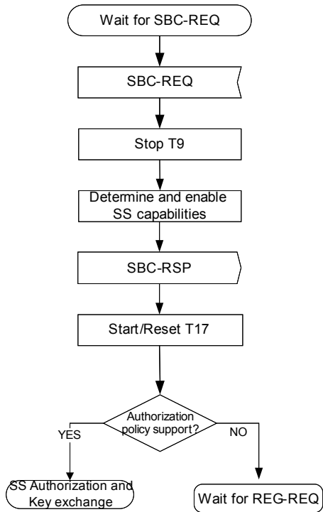
Figure 67a-Handle SBC-REQ first reception, BS side.
