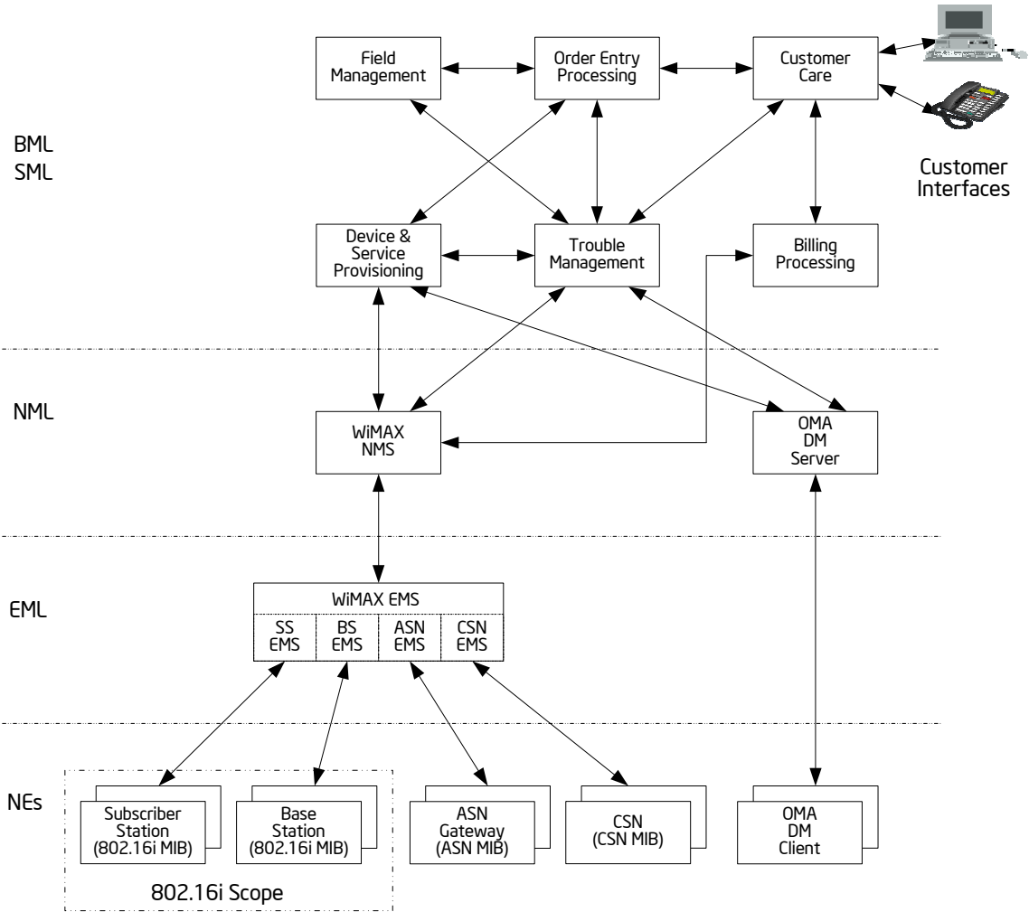
Figure 2: WiMAX OSS/BSS Reference Model
