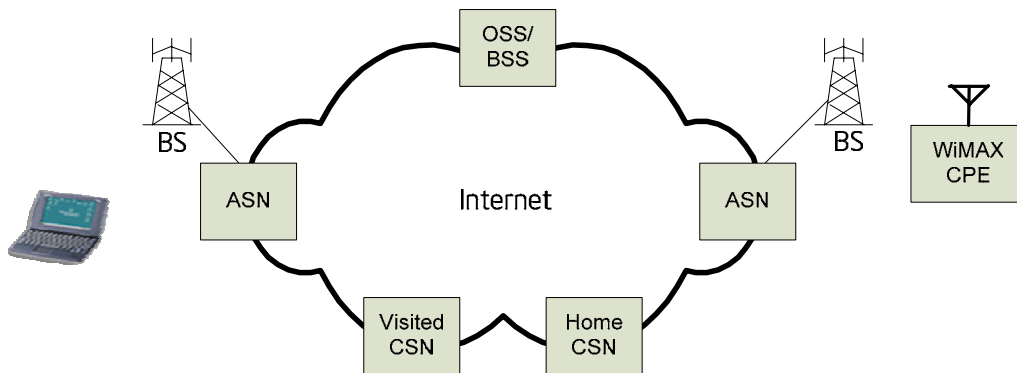
13 Figure 1: WiMAX Network Reference Model
