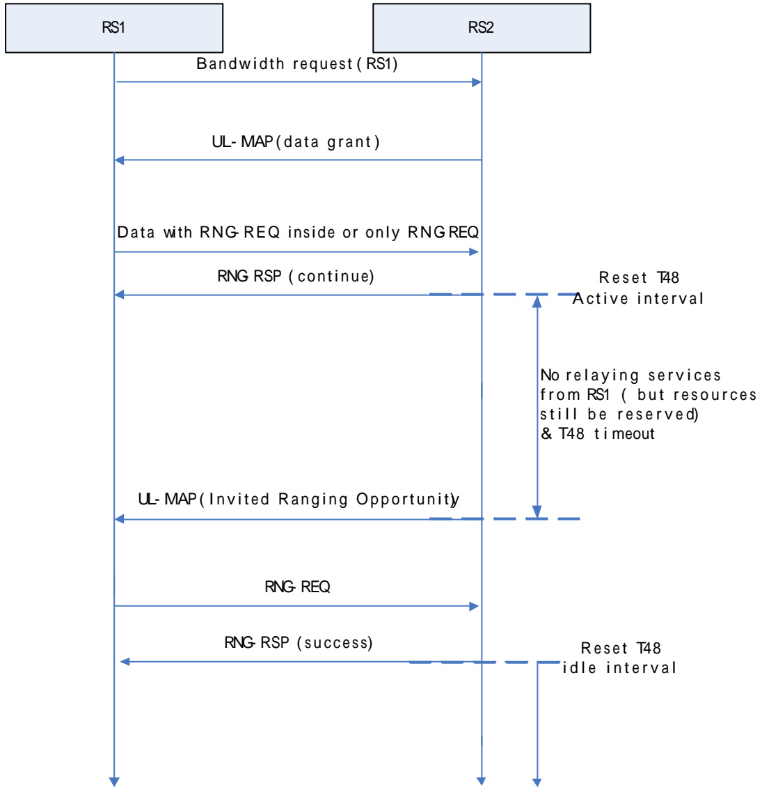
Figure 4: Periodic ranging for RS1 with separate ranging sub-channel allocation
