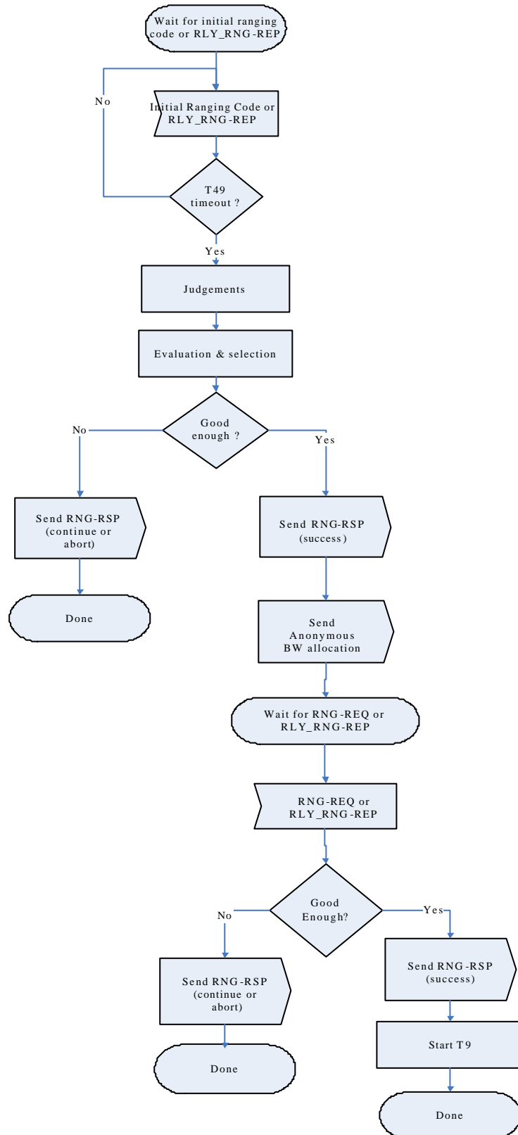
Figure E: CDMA initial ranging process with aggregate ranging sub-channel allocation (MR-BS)
