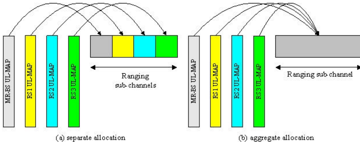
Figure 1: Two ranging sub-channel allocations
