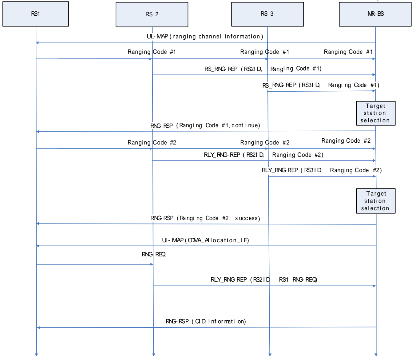
Figure 7: CDMA initial ranging process with aggregate ranging sub-channel allocation
