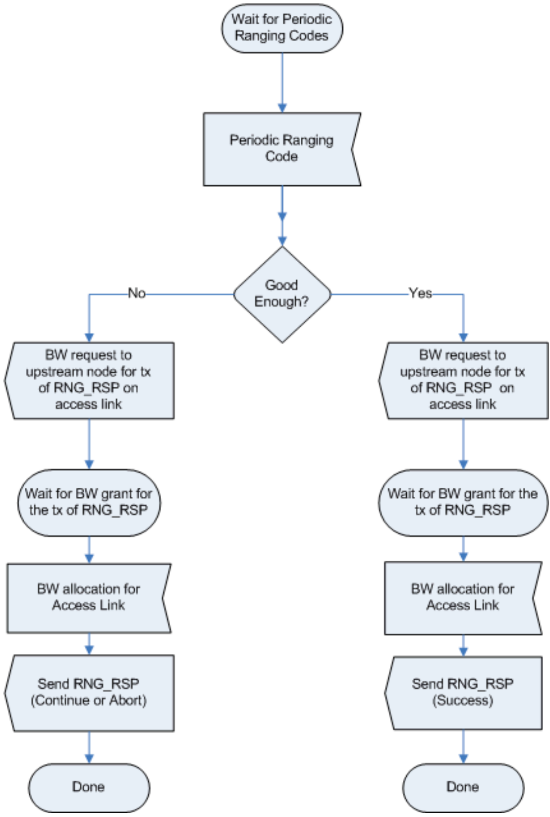
Figure 89a – CDMA Periodic Ranging – RS (centralized scheduling)
