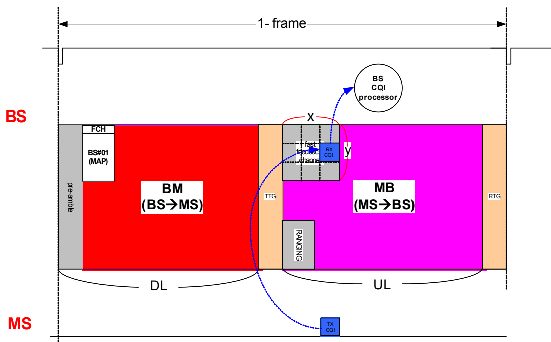
Figure 2. The example of frame structure including fast feedback channel region for OFDMA TDD system based on IEEE 802.16e standard
