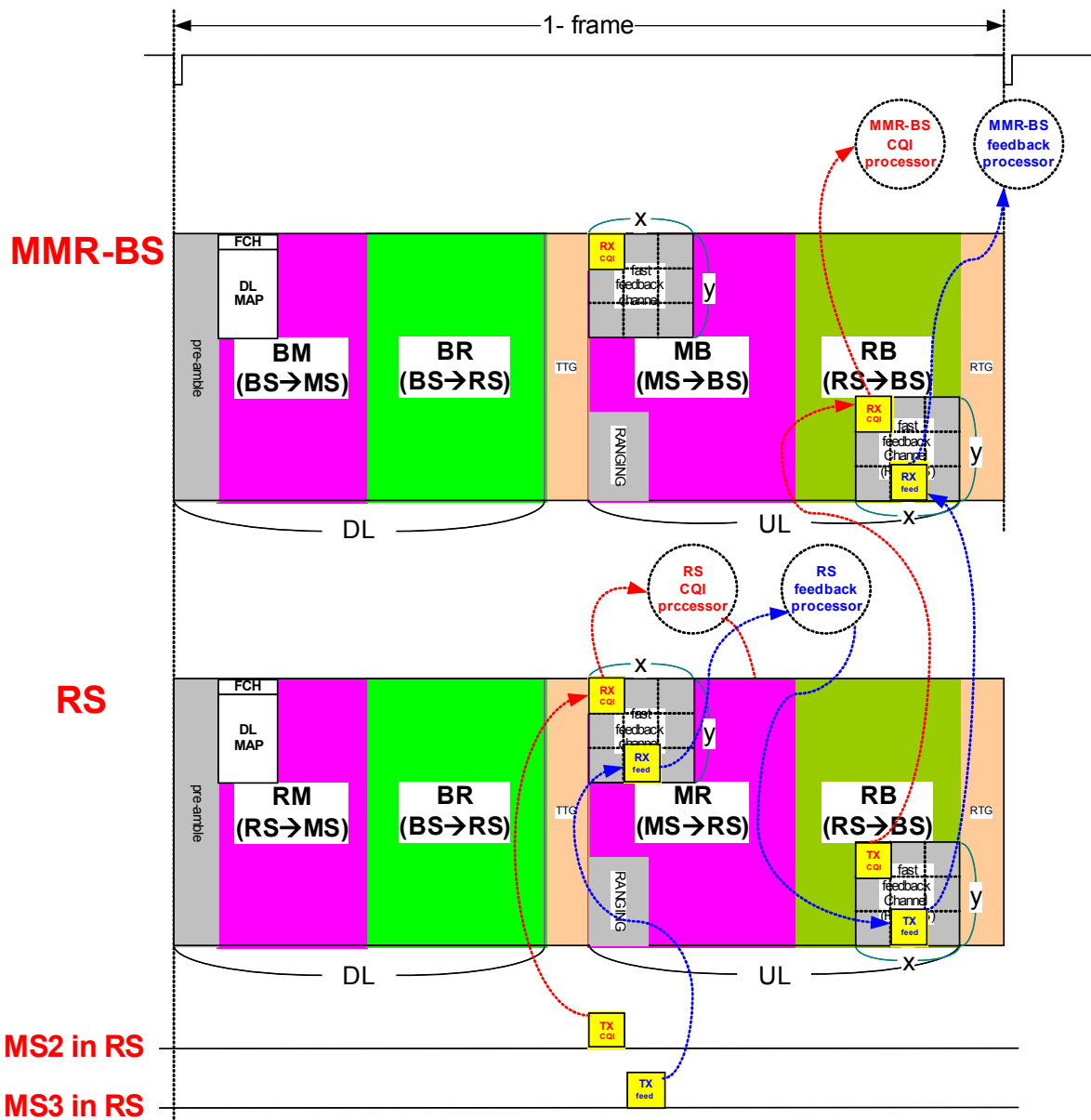
Figure 5. The example of fast feedback channel allocation in the case of using two fast feedback channel regions in a frame
