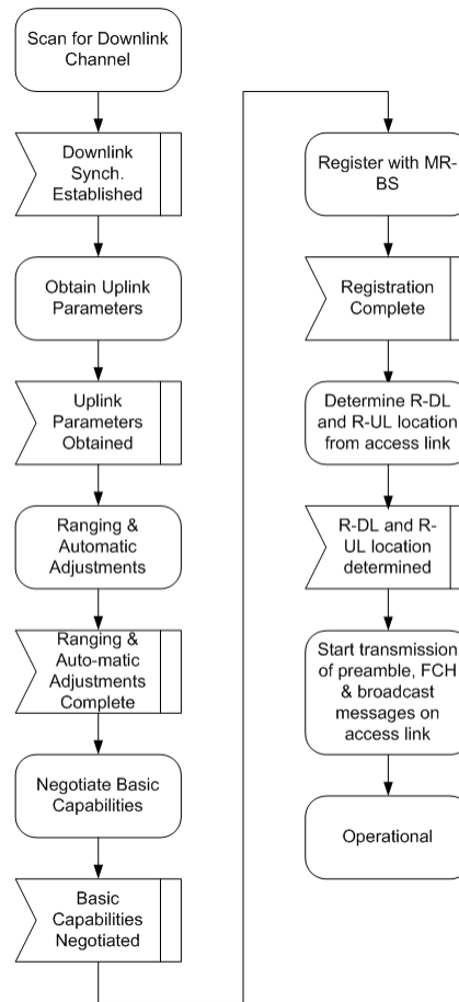
Figure 2. RS network entry procedure.
