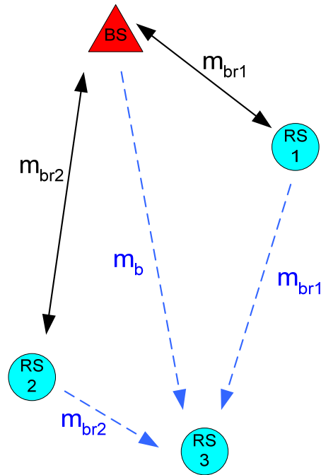
Figure 1 – RS Path metric announcement
