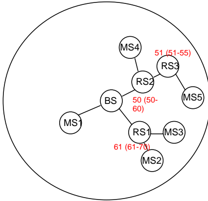
1 2 Figure 3: CID Assignment for 4.1
