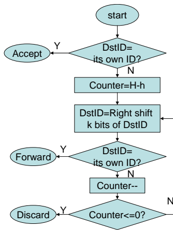
Figure 6: Subordinate RS differentiation algorithm
