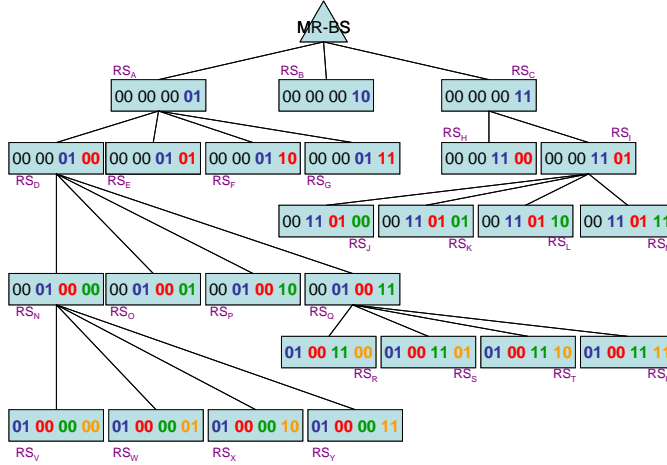
Figure 4: CID assignment for 4.2.
