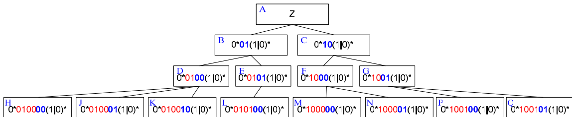
Figure 2b: partitioning of integers using bit partition.
