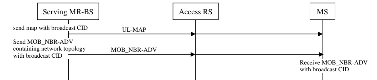
Figure xxx –Network topology advertisement in transparent RS system
