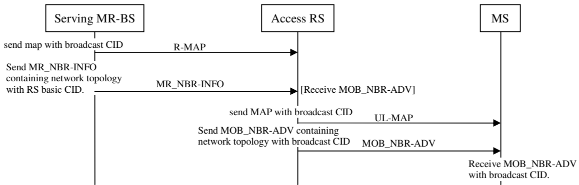
Figure zzz – Network advertisement in non-transparent RS system with distributed scheduling
