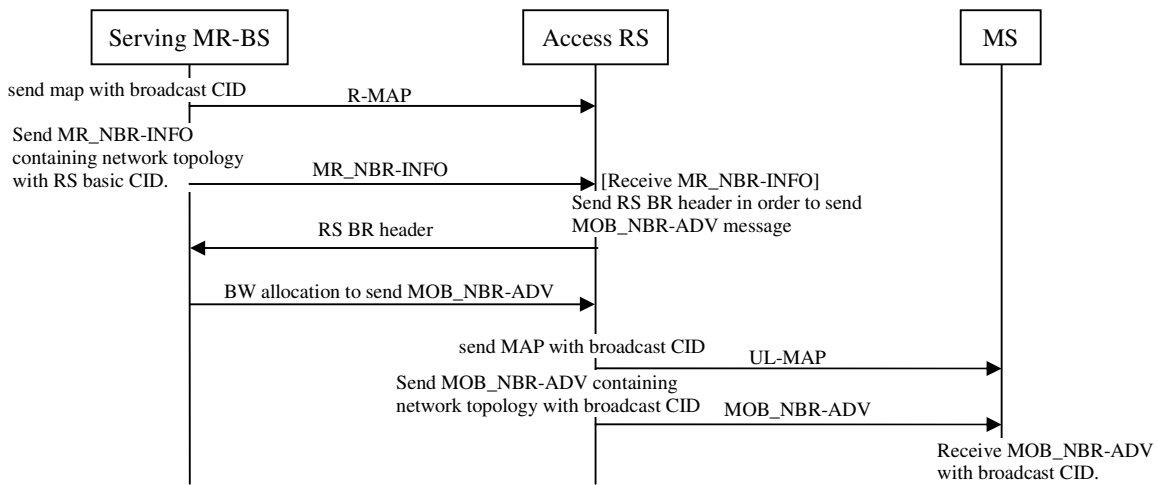
Figure yyy – Network advertisement in non-transparent RS system with centralized scheduling
