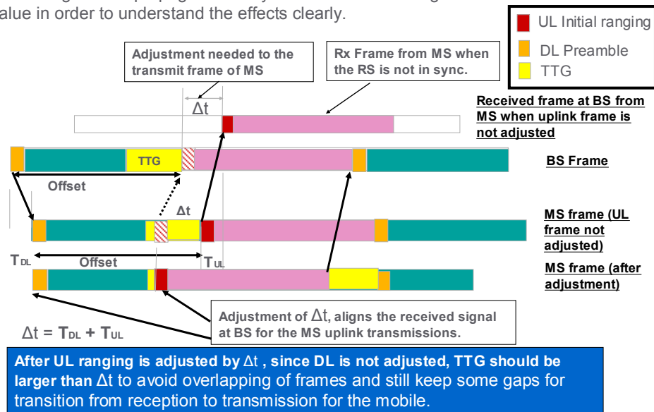
Figure 1 MS Frame alignment in 802.16e
