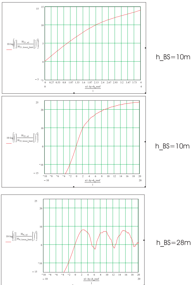
Figure 2 "Elevation gain" of a relay station above rooftop from numerical simulations. Simulation assumptions: Number of screens: 31, screen spacing: 50 m, frequency: 2 GHz, screen height: 8m.
