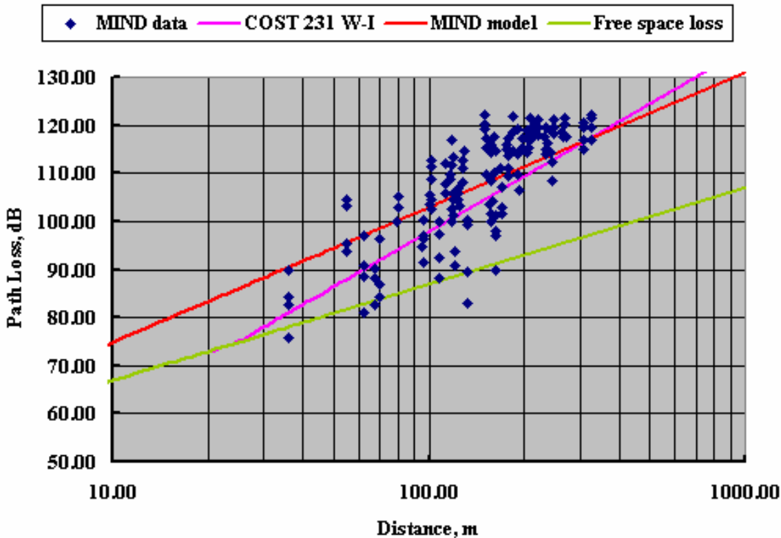
Fig. 3 comparison of the modified COST 231 W-I model with the measured data from IST MIND, and the IST MIND empirical path loss model b = 50\text{m} ; w = 30\text{m} ; h_r = 6.5\text{m} ; h_b = h_m = 8\text{m} ; f = 5.3\text{GHz}
