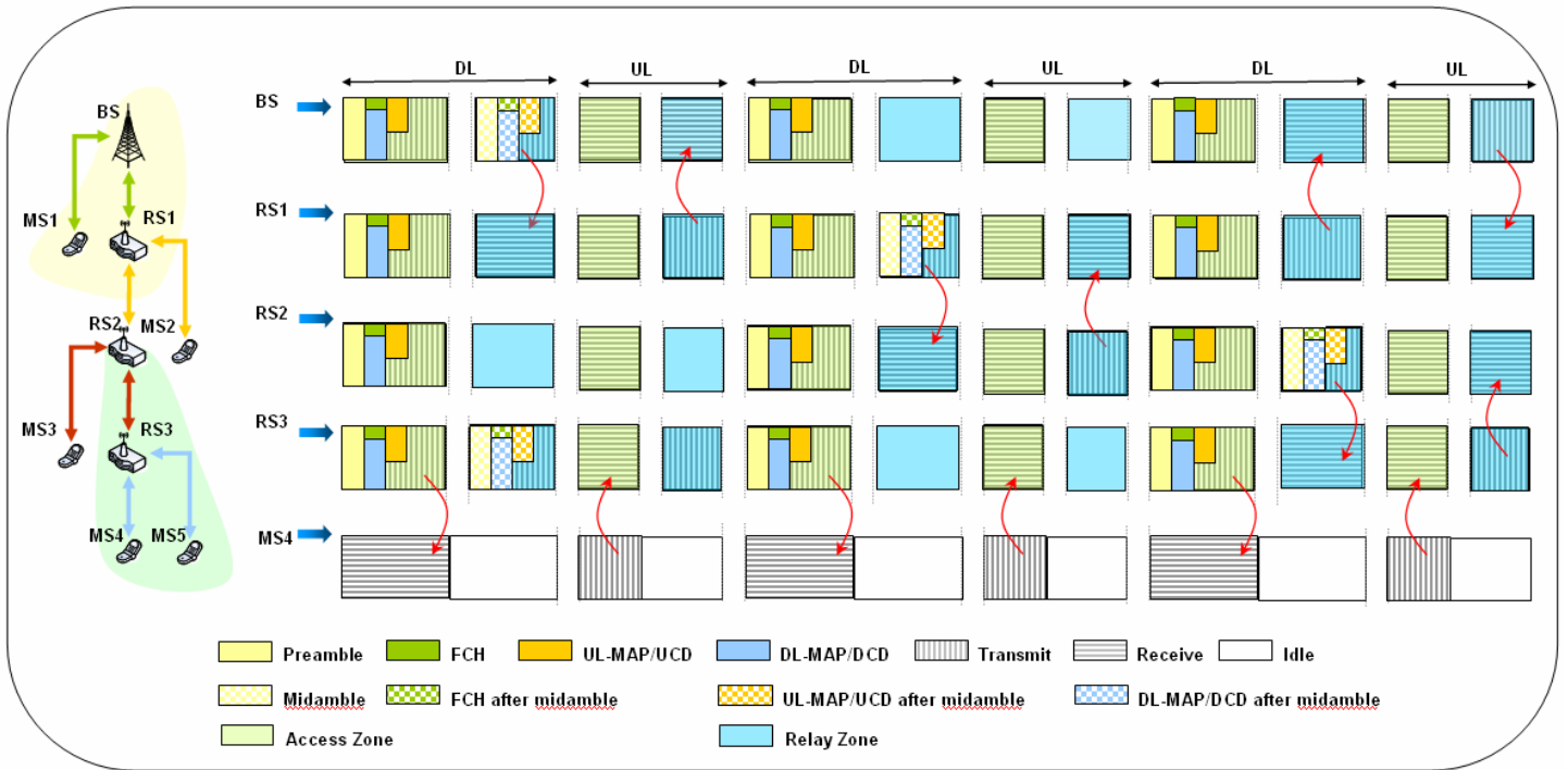
Figure 3: A super frame with single relay zone in each DL and UL sub-frame – one transmission in each super frame
