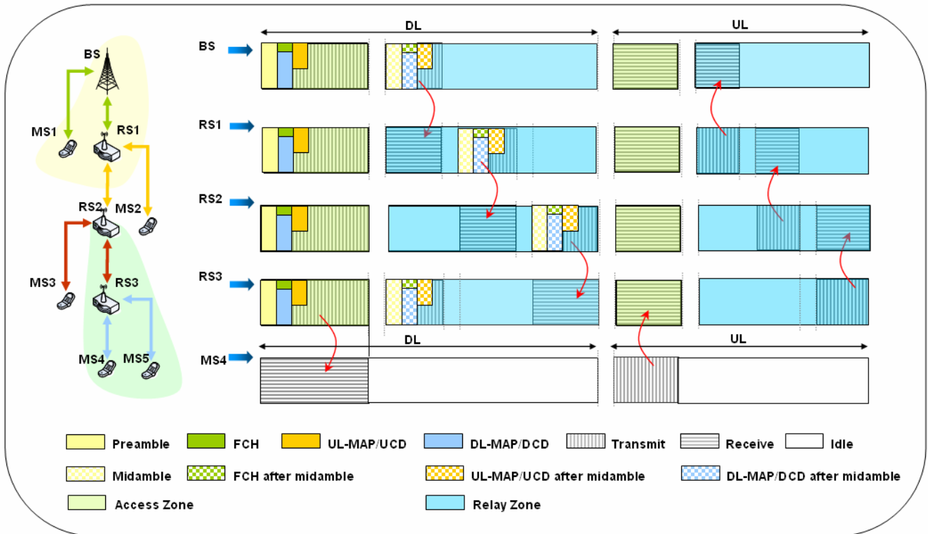
Figure 2: Frame structure with more than one relay zone in the DL and UL sub-frames
