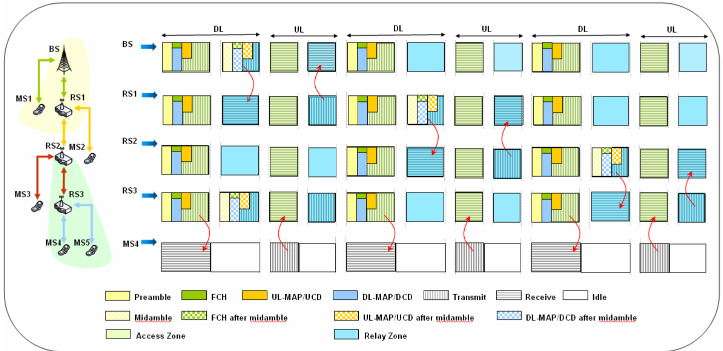
Figure 4: A super frame with single relay zone in each DL and UL sub-frame – multiple transmissions in each super frame where interference impact is negligible
