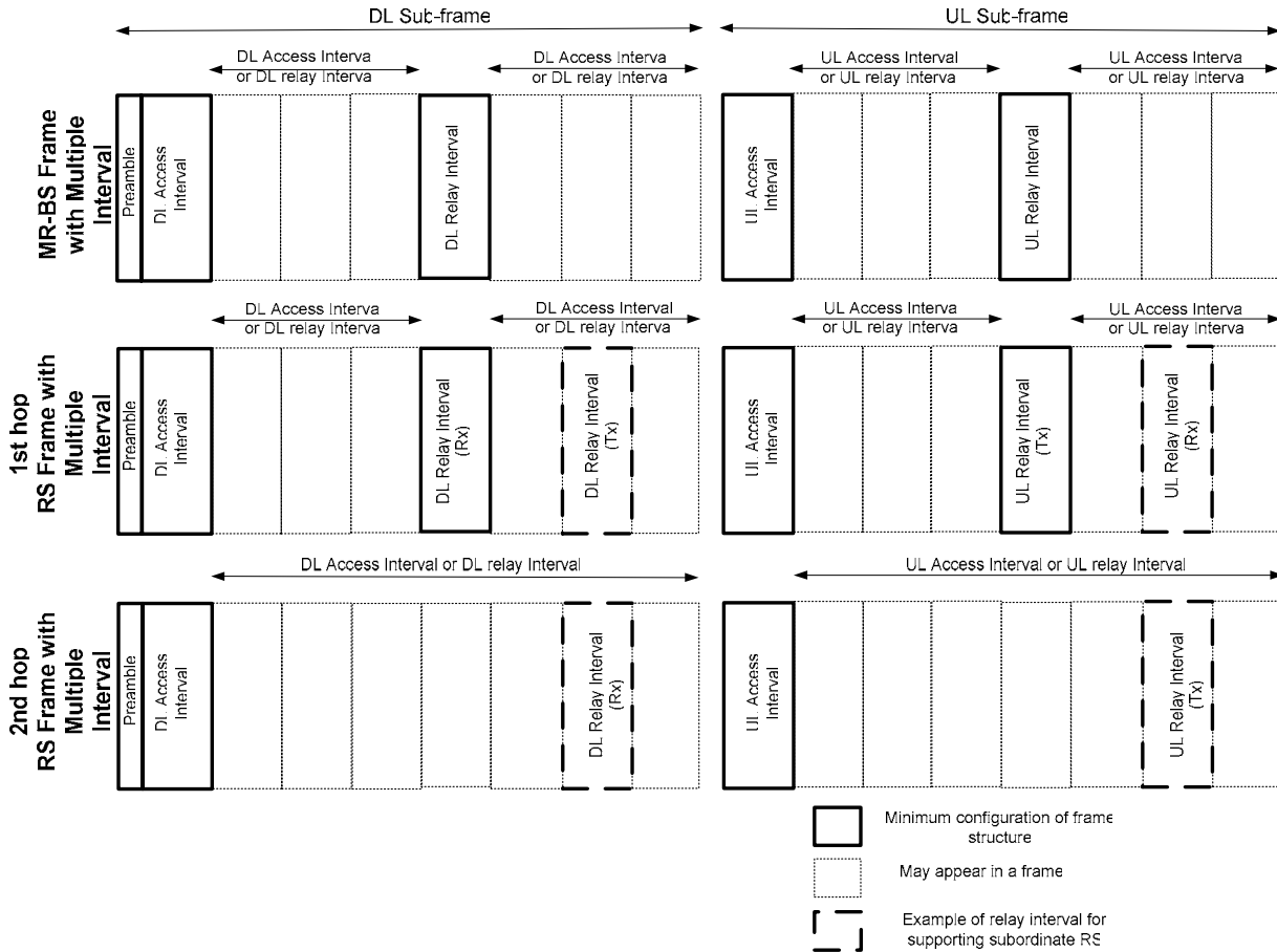
Figure zzz Relay frame with multiple intervals
