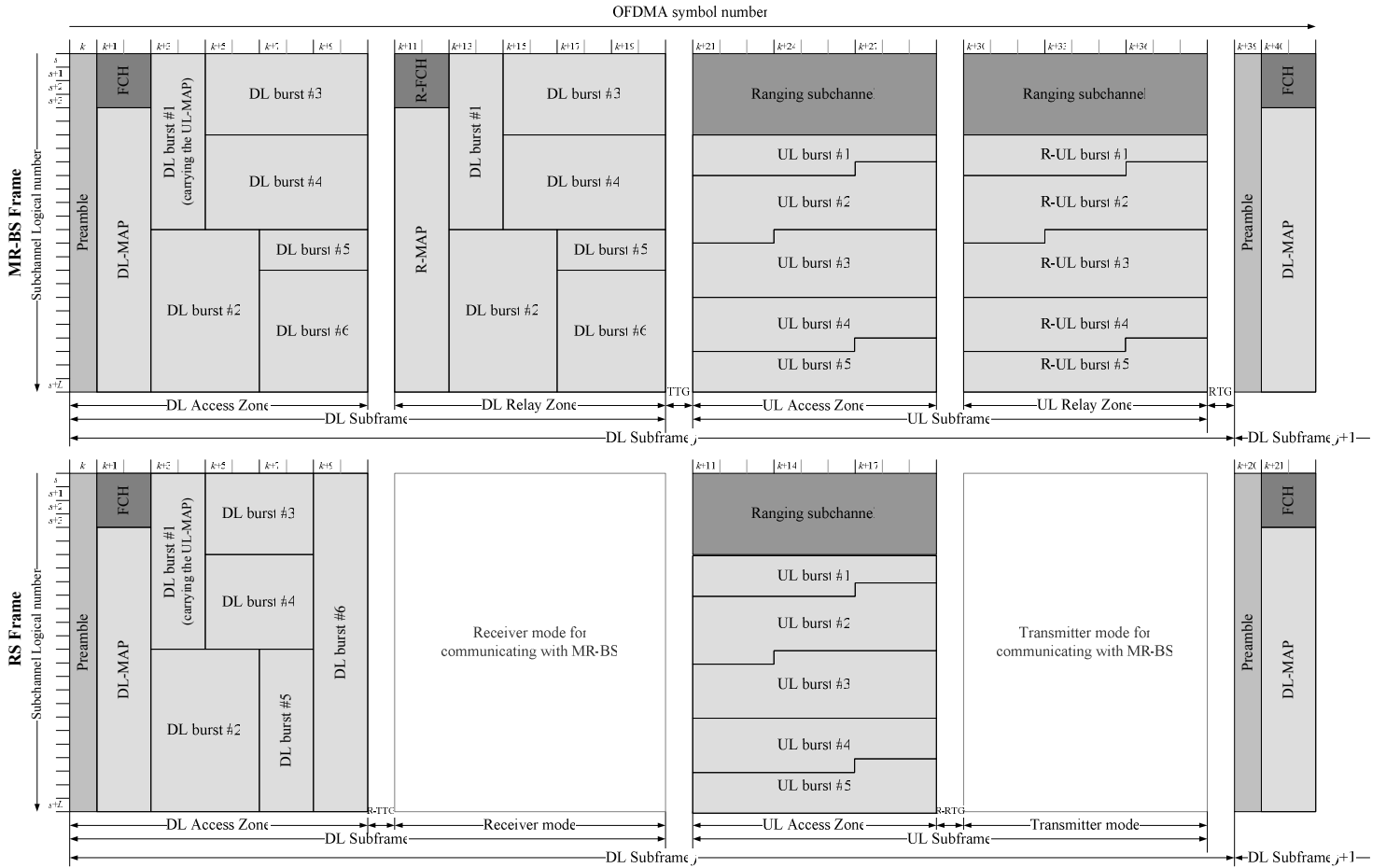
Figure yyy —Example of minimum configuration for an in-band non-transparent relay frame structure
