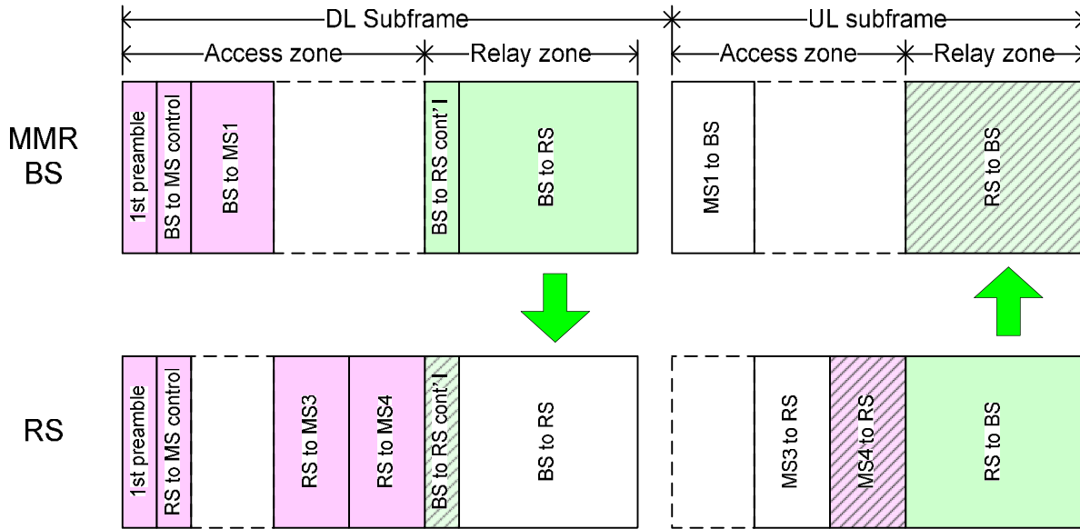
Figure 5 Modified frame structure (three MSs)
