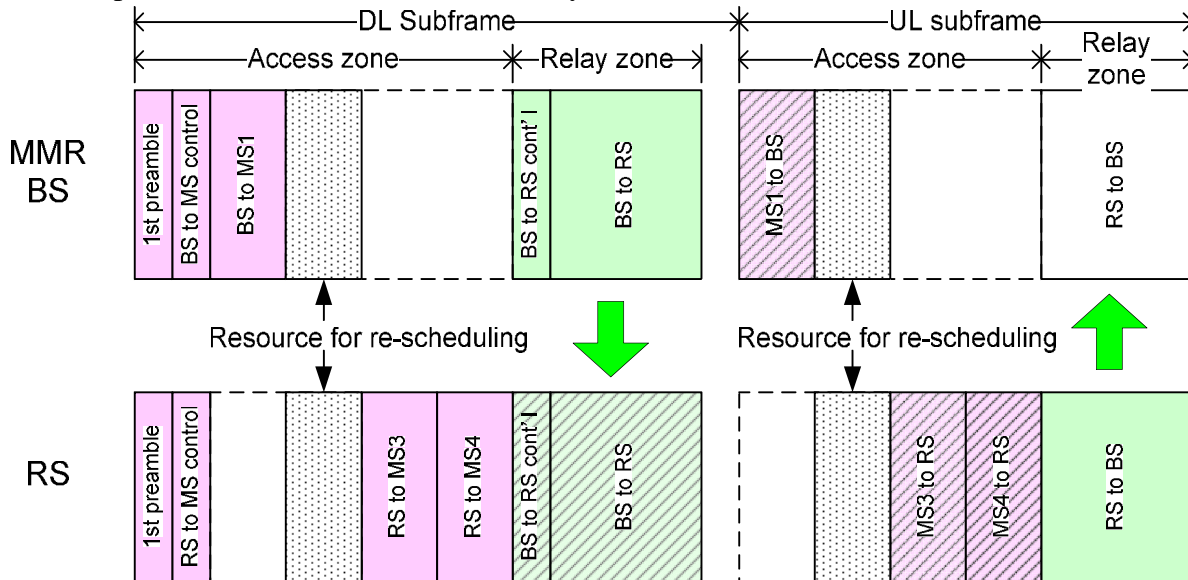
Figure 4 Expected frame structure
