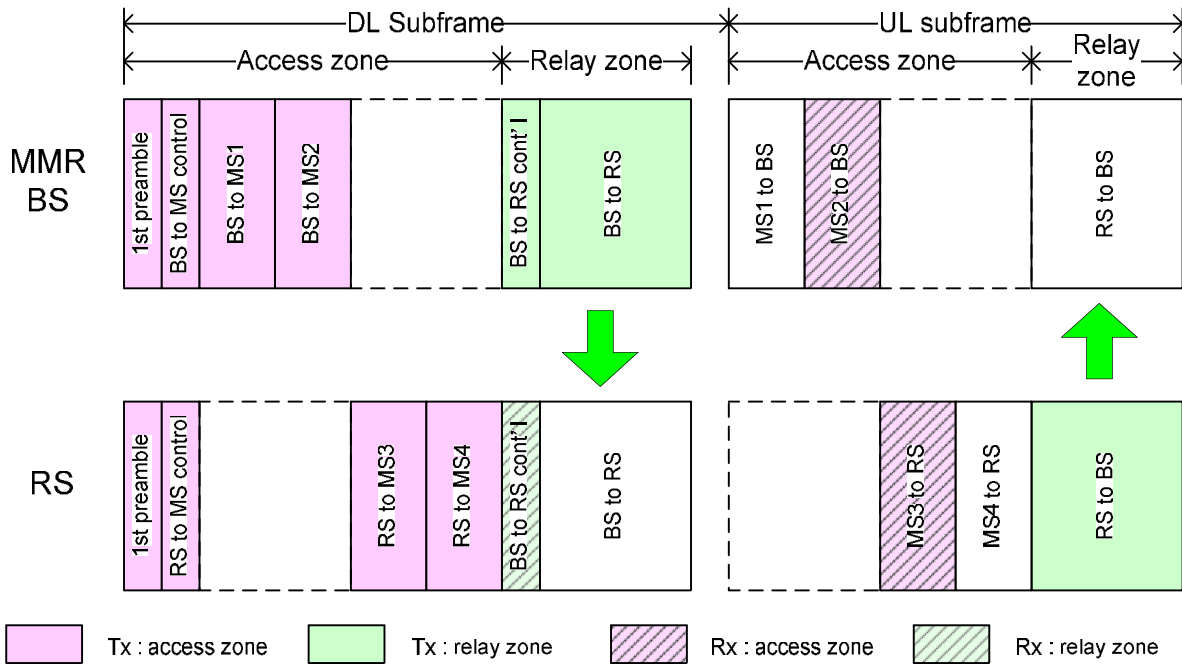
Figure 2. Frame structure example
