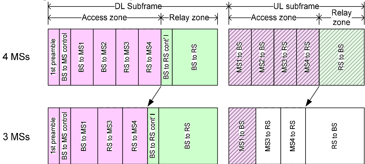
Figure 6 Comparison of zone boundary for 3 MS case and 4 MS case (superimposed)
