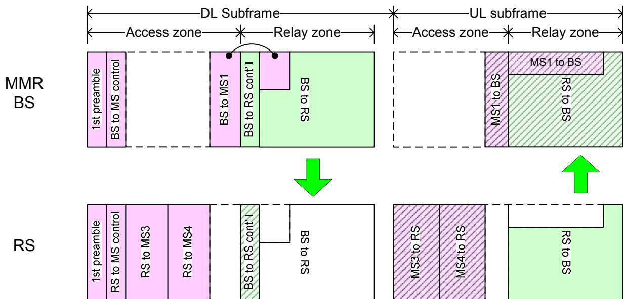
Figure 8. Frame implementation example for Figure 3.
