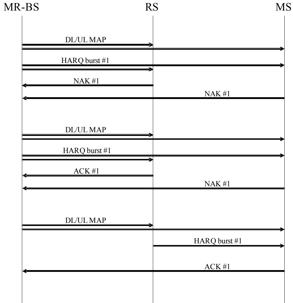
Figure 3 RS-assisted relaying
