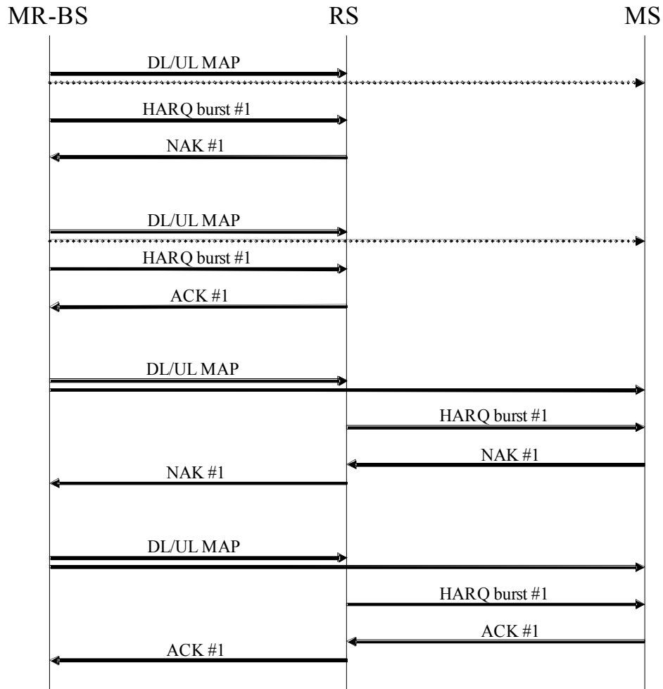
Figure 2 Hop-by-Hop relaying
