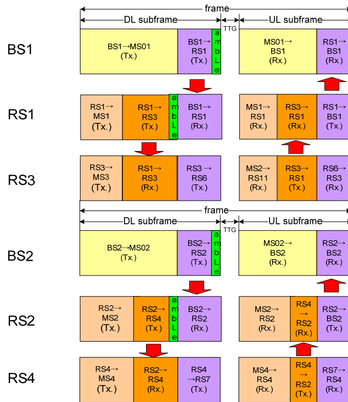
Figure 3 An example of frame structure with amble at the end of DL relay zone.
