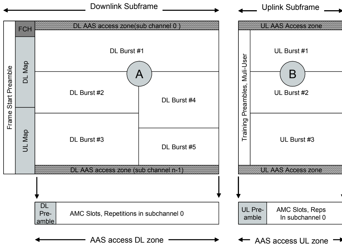
Figure 5. AAS Relay Zone Frame Structure
