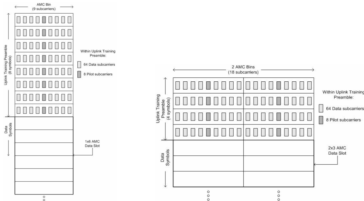
Figure 6. AAS Preamble Construction using 1 x 6 and 2 x 3 AMC Bins
