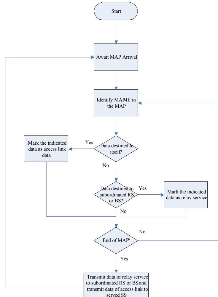
Figure xxx – Relay Service Flow Chart of RS
