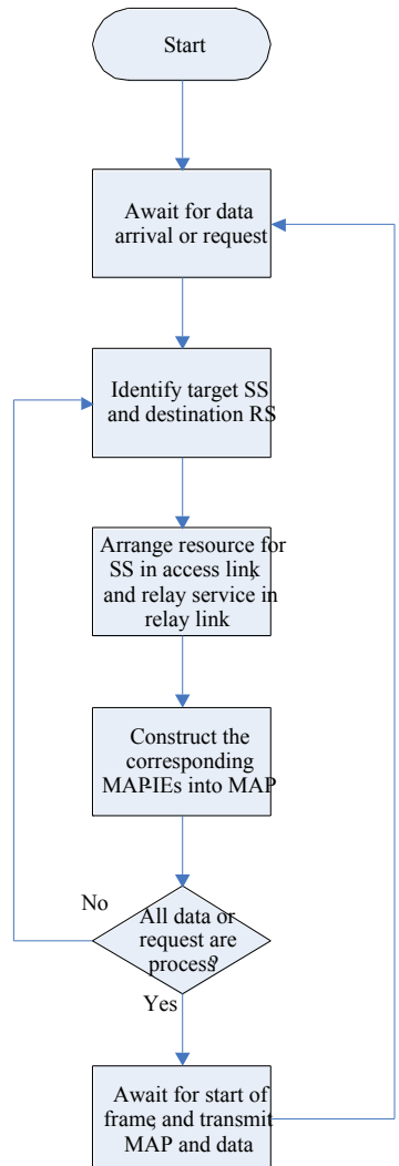
Figure xxx – Relay Service Flow Chart of MR-BS
