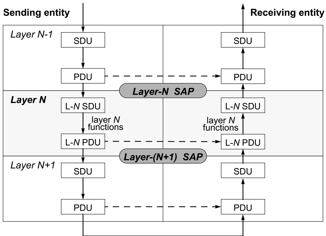
Figure 3: PDU vs. SDU in a protocol stack.
