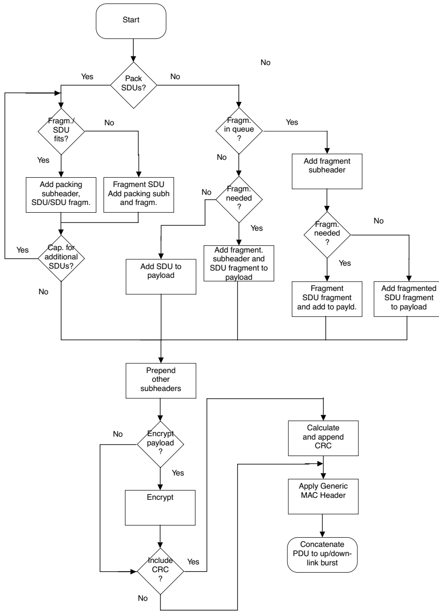
Figure 1—Construction of a MAC PDU
