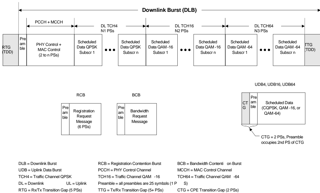
Figure 5-5 Types of Bursts
