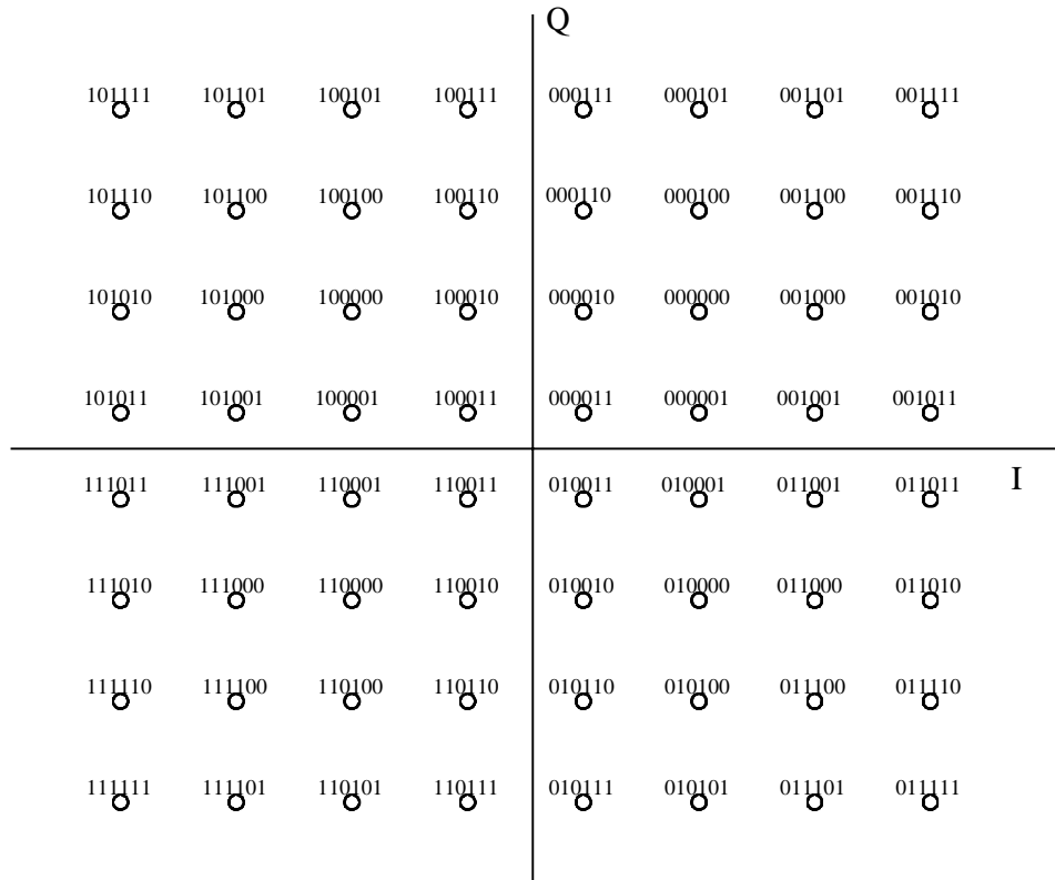
Figure 7-3 QAM-64 Constellation
