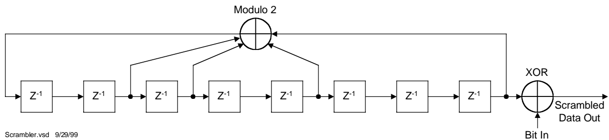
Figure 6-2 Scrambling Sequence Generator
