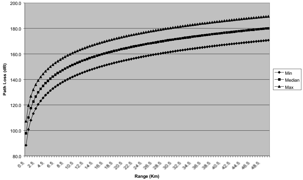
Figure 248a Path Loss Model for 30 m Base Station antenna height (for Category C).
