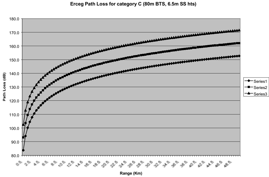
Figure 248b Path Loss Model for 80 m Base Station antenna height (for Category C).
