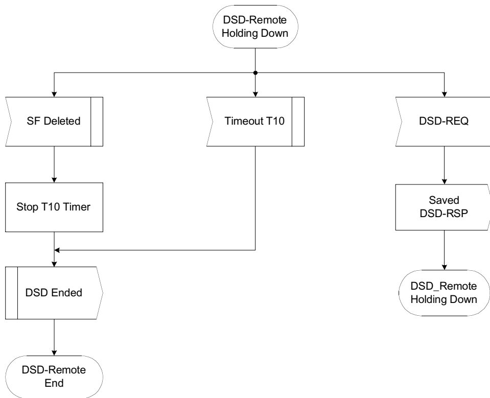
Figure 97 DSD — Remotely Initiated Transaction Holding Down State Flow Diagram
