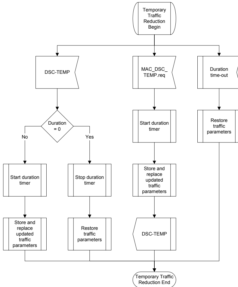
Figure 125 - DSC-TEMP mechanism
