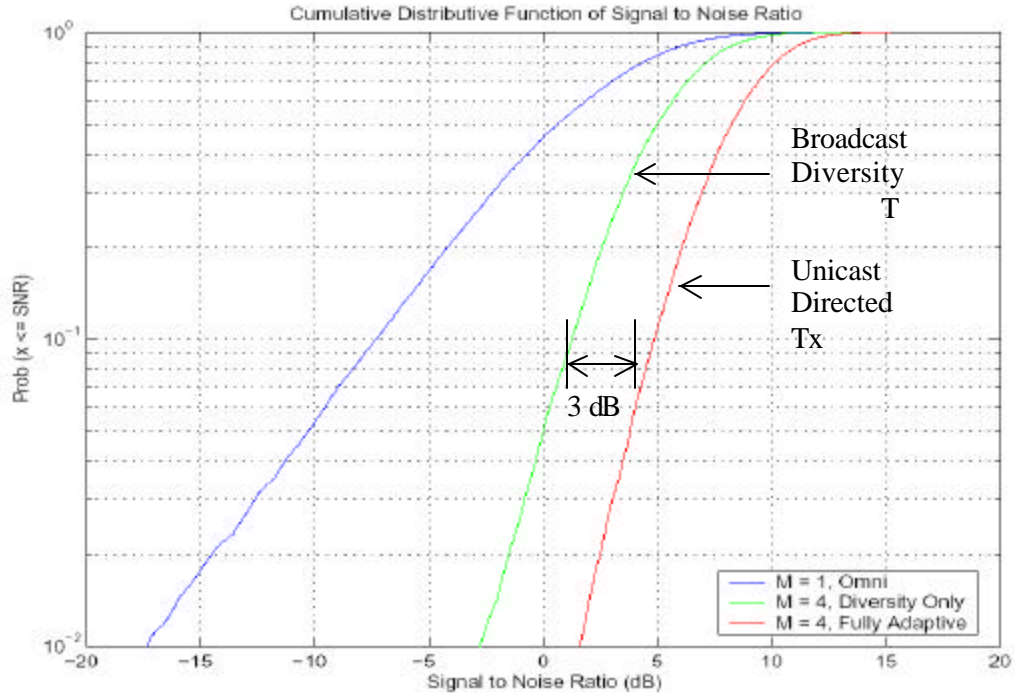
Figure 4: Downlink SNR Distribution for a cell-edge user on the broadcast and directed transmissions.
