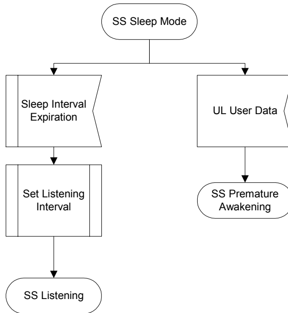
Figure 123c—SS Await Poll SDL Diagram
