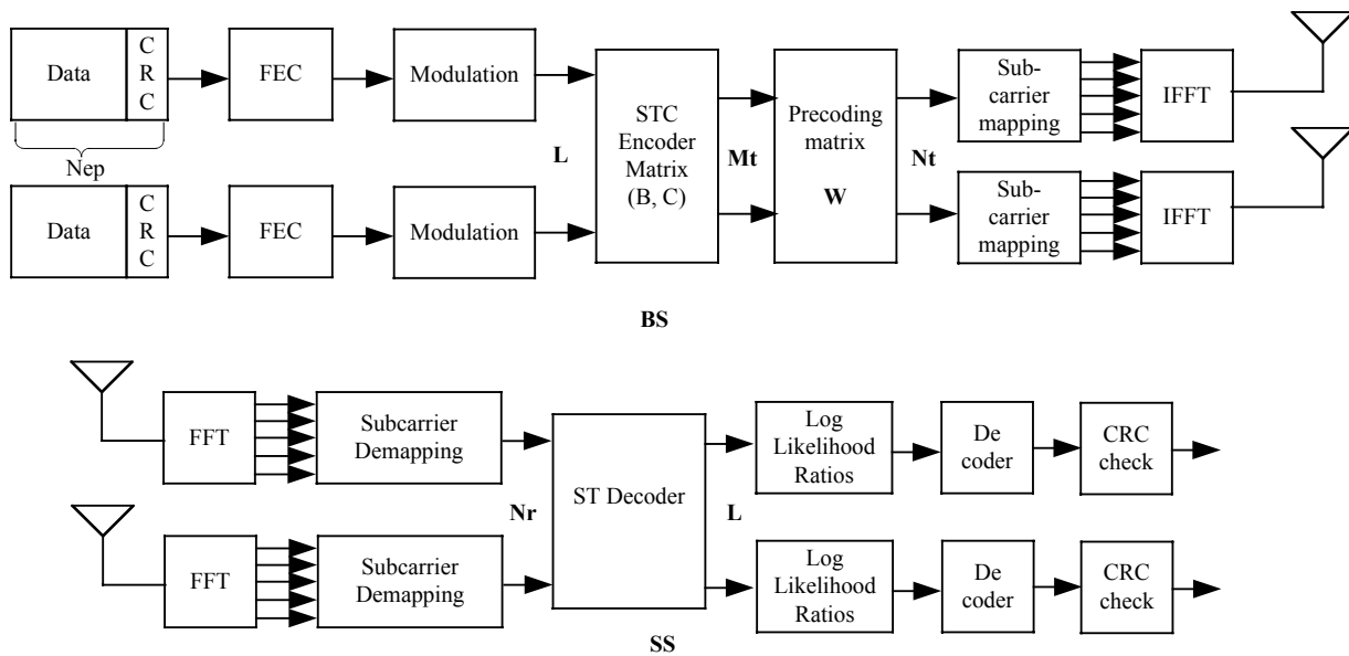
Figure 2 H-ARQ Enabled Horizontally Encoded 2x2 MIMO System
