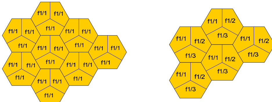
14 15 (a) Full re-use 1 identical segments (1,3,1/1)
