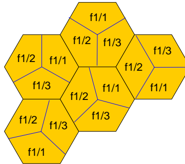
10 11 12 Figure 9.5: Frequency reuse pattern on preamble sub-carriers for Scenario I with different 13 segment numbers in case of spatially unplanned antennas. 14
