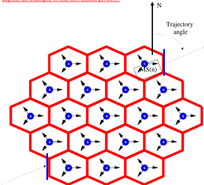
Figure 3. - 19 cell abbreviated example of MS movement in a wrap around environment. Blue lines denote paired wrap around boundary segment.
