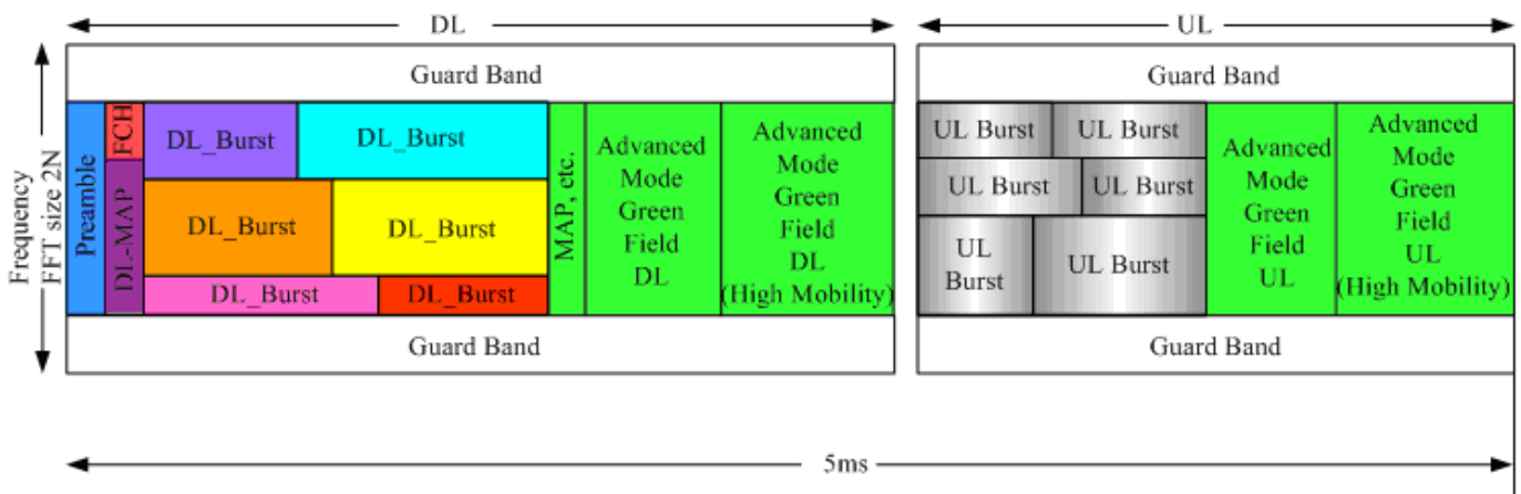
Figure 1. OFDMA frame structure for IEEE 802.16m with high-mobility support
