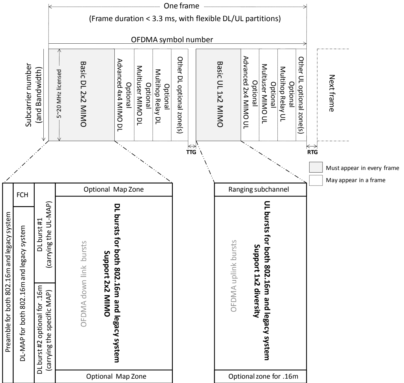
Figure 1: Frame structure for basic and advanced feature
