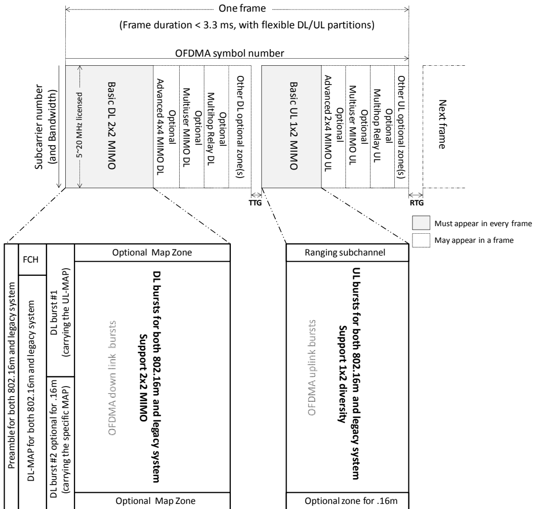
Figure aaa – Example of an OFDMA frame with basic zone (mandatory zone) in TDD mode
