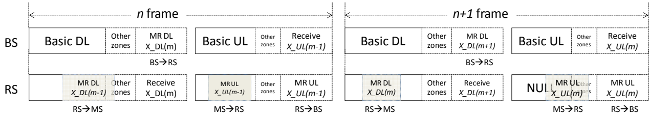
(b) with radio resource reuse
