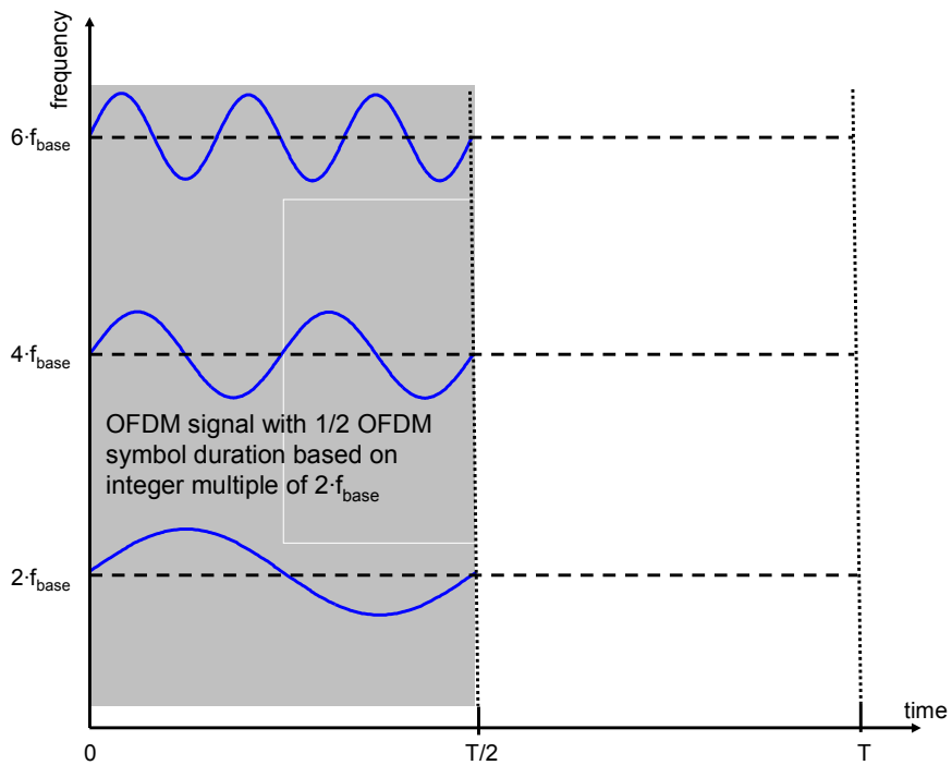
Figure 9: Even Integer Multiple of Base Frequency for Fractional Symbol Time OFDM Signal
