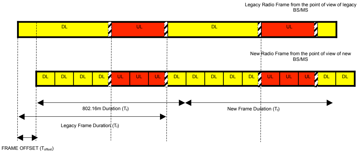
Figure 11.4-3: Relative position of the new and legacy radio frames (example TDD duplex scheme) → proposal-1
