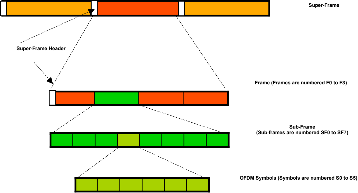
20 21 22 Figure 11.4-1: Basic frame structure
