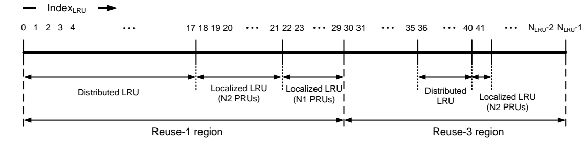
Figure 4 – Example of LRU indexing for different resource types.
