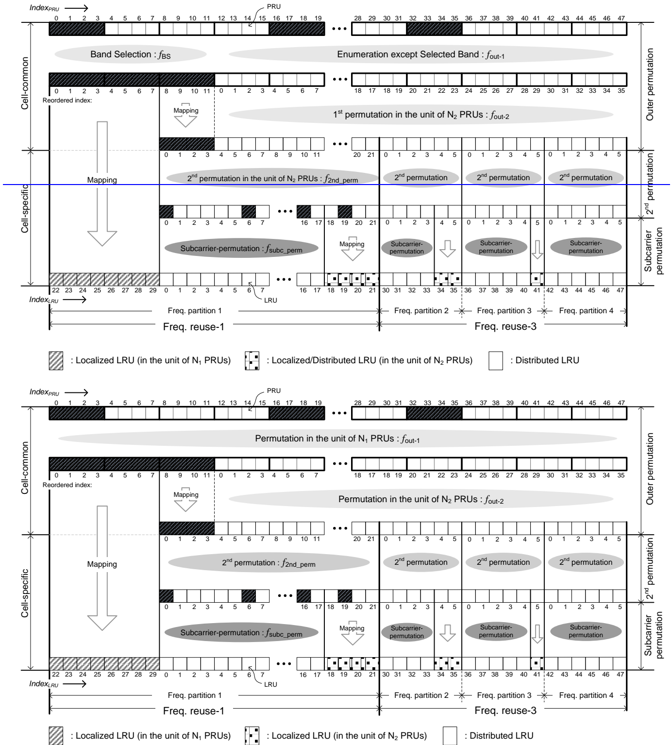
Figure 2 – Detailed description of downlink subcarrier to resource block mapping (BW=10MHz, N_1=4 , N_2=1 )
