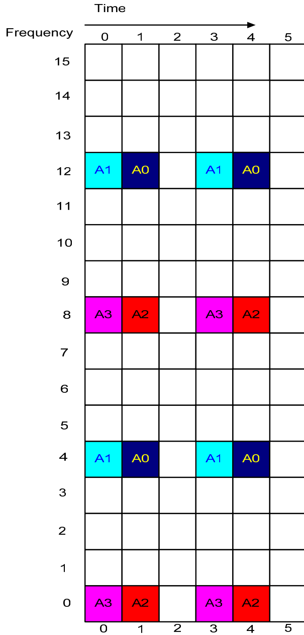
Figure 1 Pilot patterns per slot.
