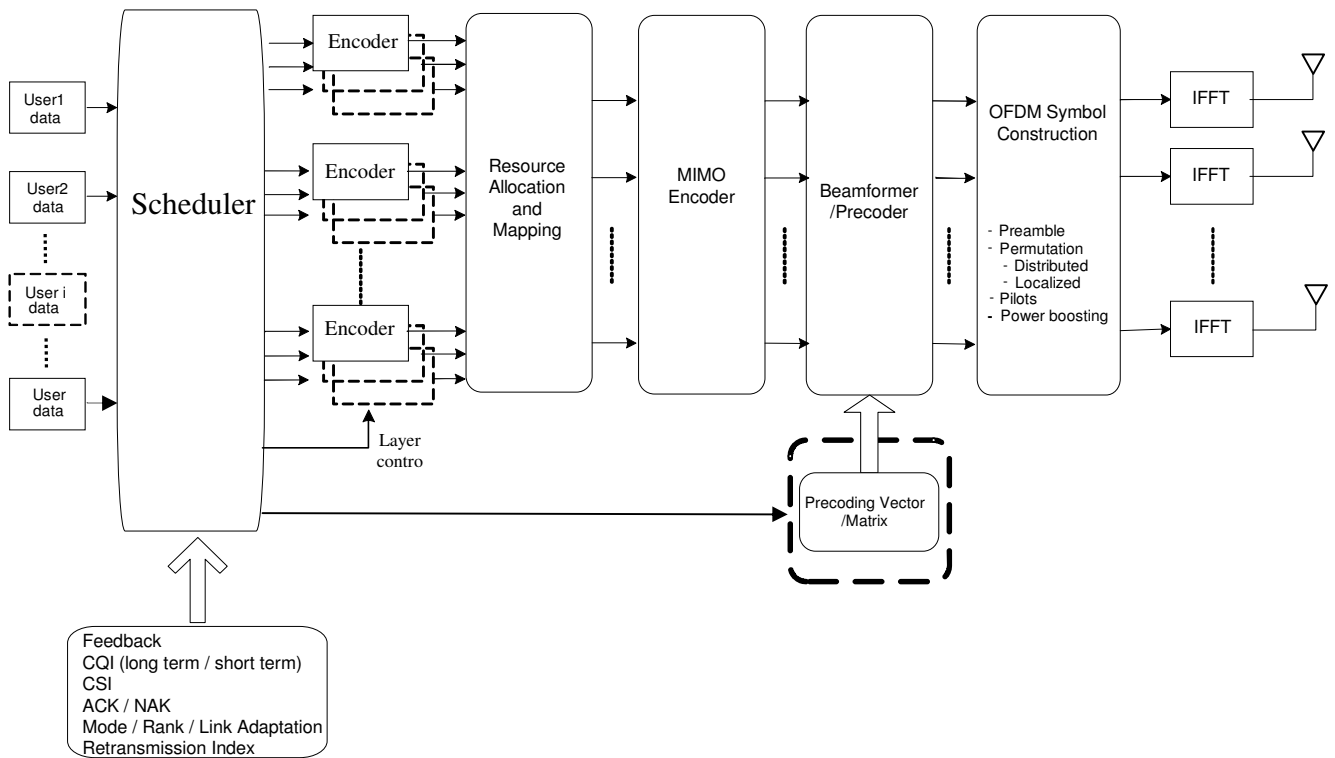
Figure 1: MIMO Architecture
