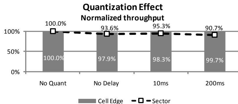
Figure 5. Effect of feedback quantization on the proposed technique
