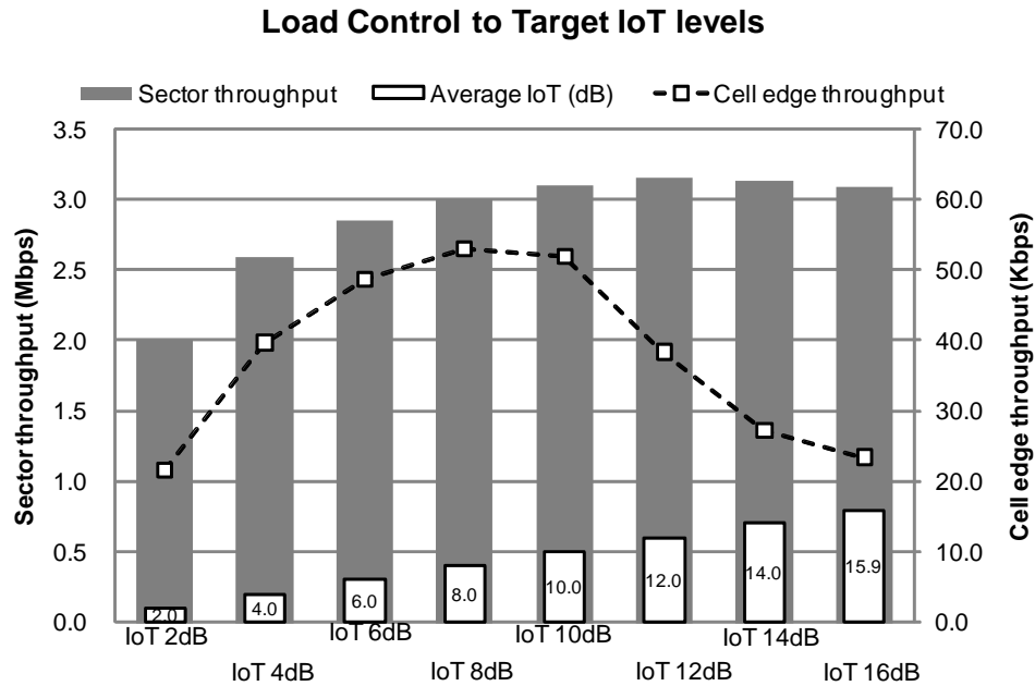
Figure 4. System performance along with target IoT level
