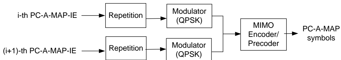
Figure 9. Block diagram of PC-A-MAP IE to PC-A-MAP symbols
