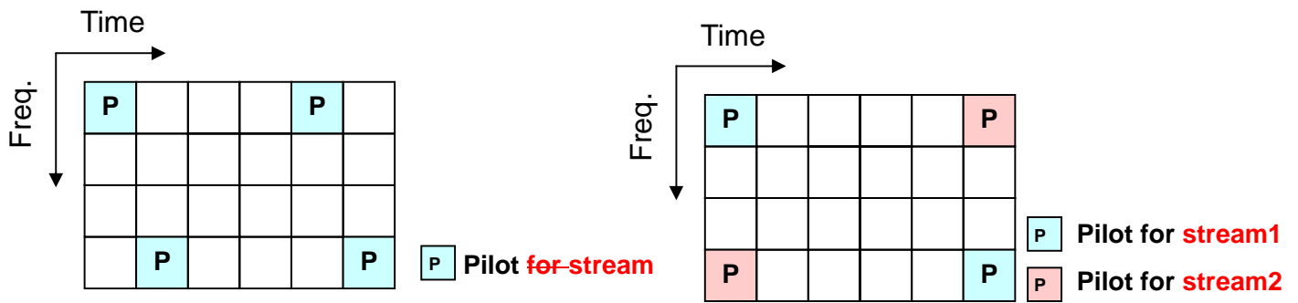
Figure 1 Tile structure in 16m PUSC
