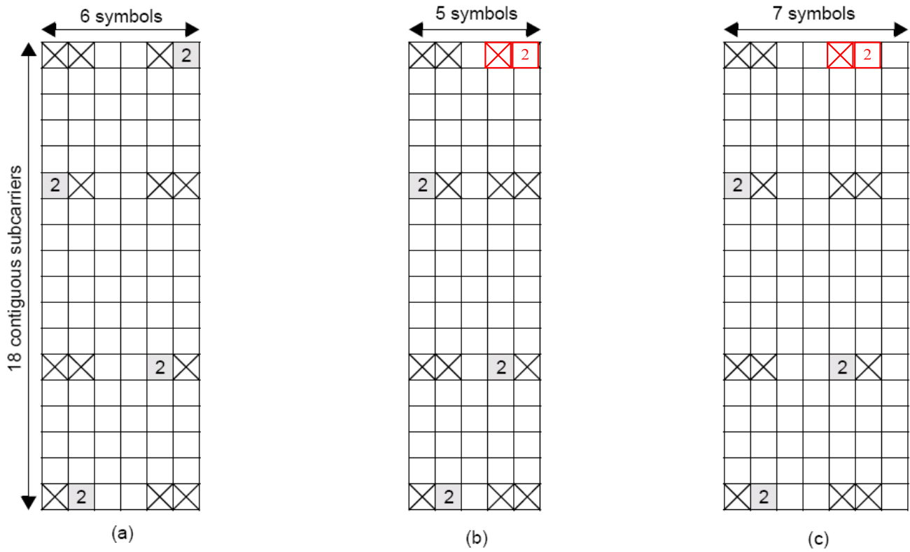
Figure 459—Pilot patterns on stream 1 for 4 data streams
