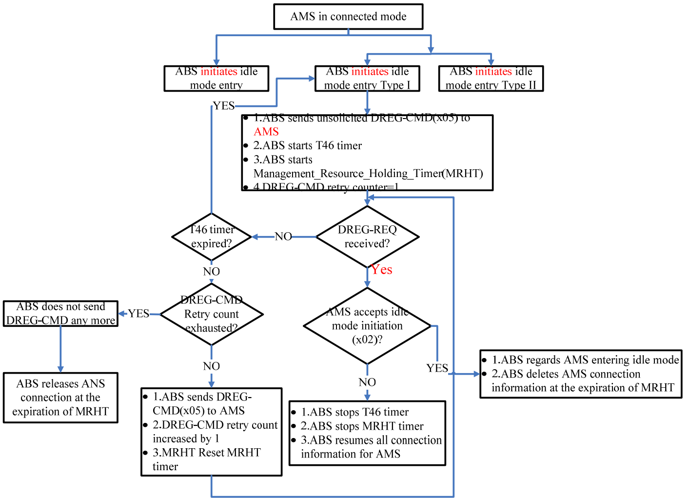
Figure 419—Procedures during Type I ABS initiates idle mode entry
