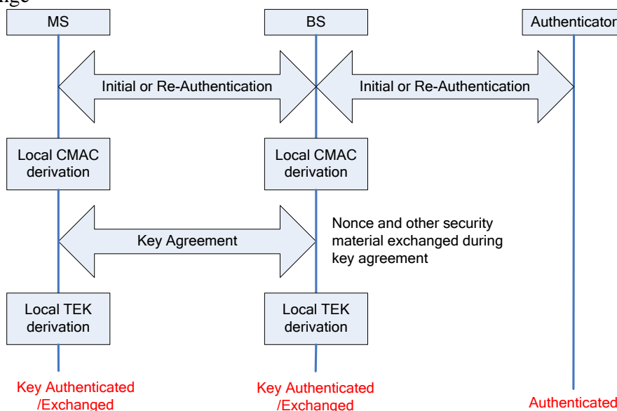
Figure 18 Initial or Re-authentication – Key Derivation and Exchange
