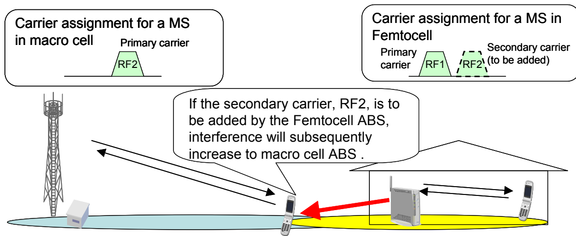
Fig.2 Illustration of the scenario of interference increase in multi-carrier operation for Femtocell ABS.
