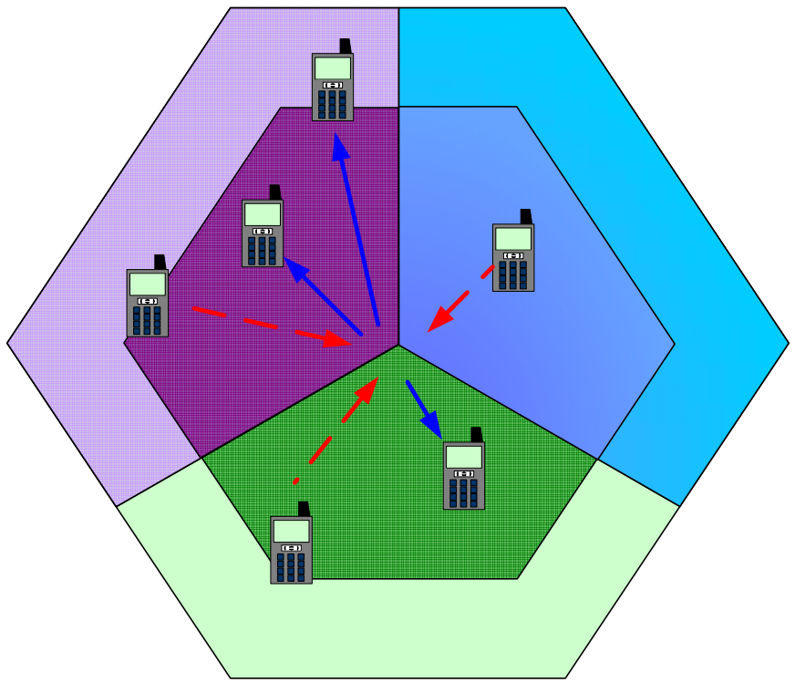
Data Transition Interference in TDD
