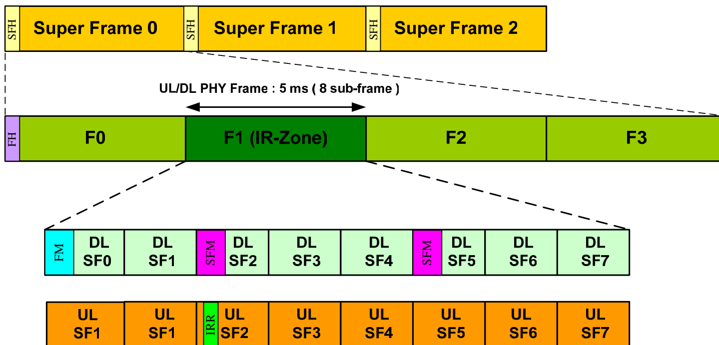
Control channel structure for FDD
