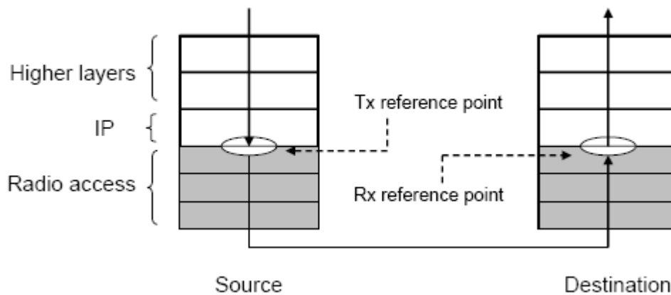
Figure 1-Illustration of reference points for the user-plane data latency
